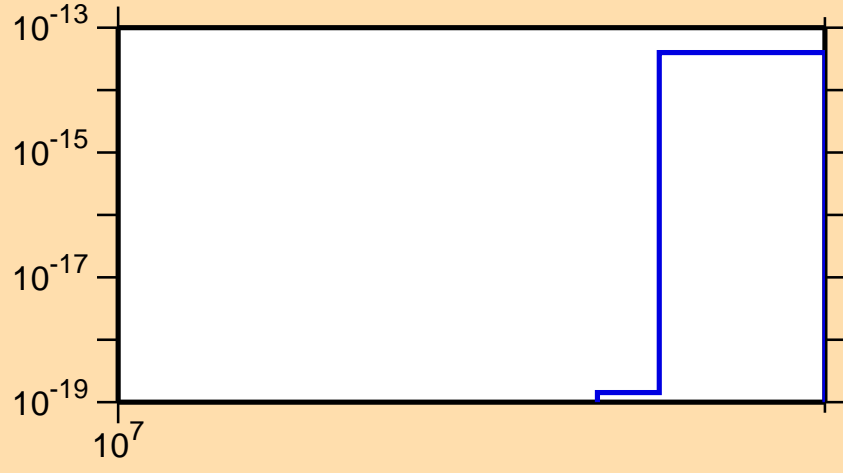
\sigma vs. E for ^{154}\text{Pm}(n,\text{He}3)
