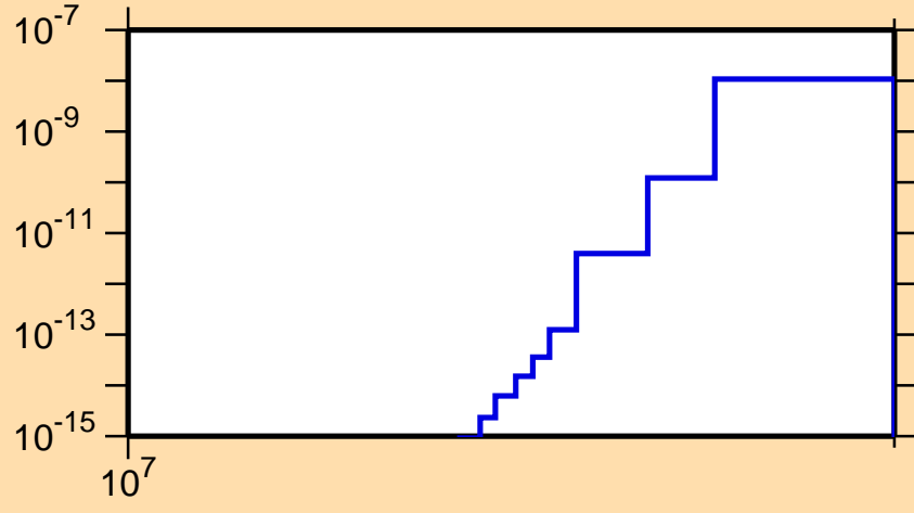
\sigma vs. E for ^{154}\text{Pm}(n,2n\alpha)
