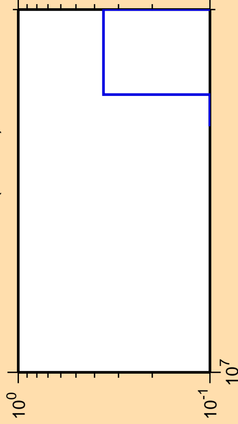
\Delta\sigma/\sigma vs. E for ^{154}\text{Pm}(n,\text{He}3)
