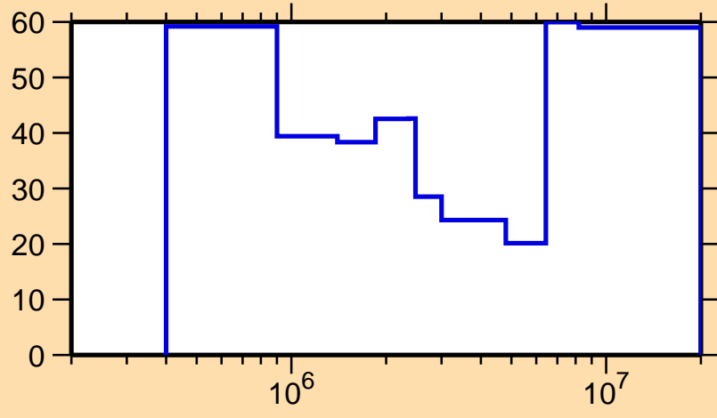
\Delta\sigma/\sigma vs. E for ^{154}\text{Pm}(n,n\text{cont.})
