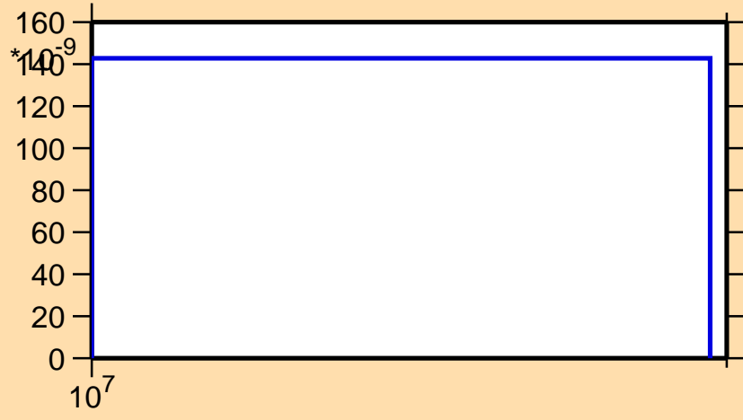
\sigma vs. E for ^{154}\text{Pm}(n,nd)
