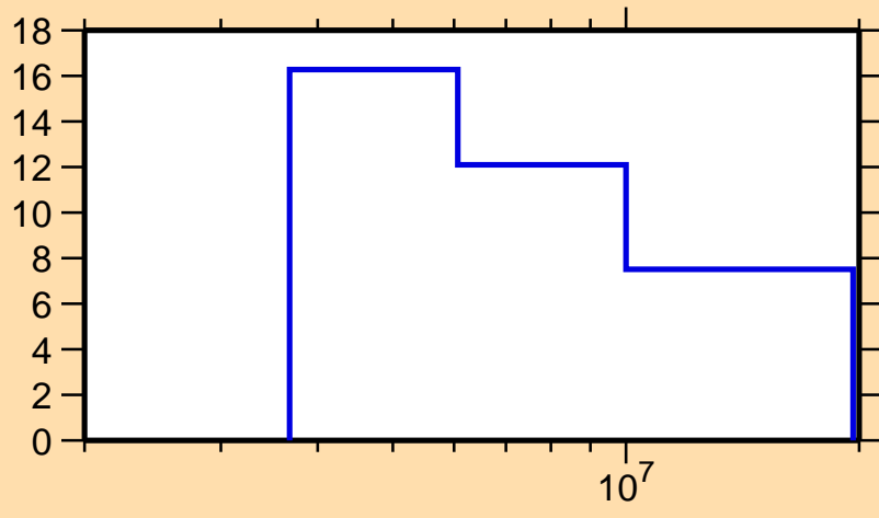
\Delta\sigma/\sigma vs. E for ^{155}\text{Pm}(n,\text{tot.})
