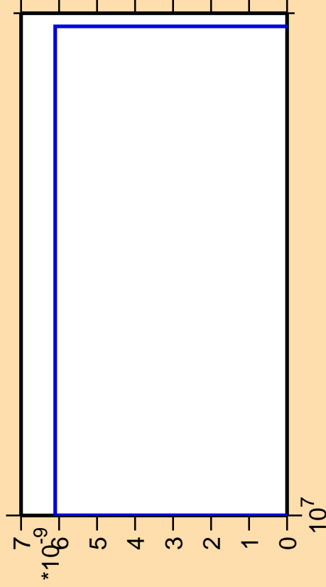
\Delta\sigma/\sigma vs. E for ^{155}\text{Pm} (mt 11)
