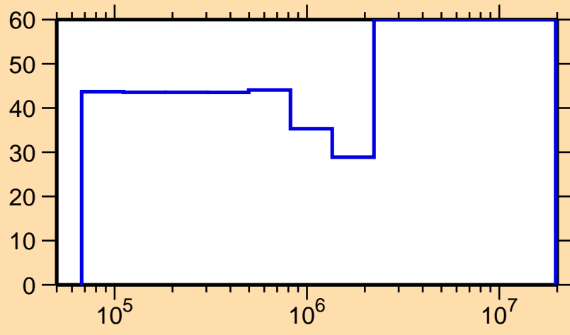
\Delta\sigma/\sigma vs. E for ^{155}\text{Pm}(n,n_1)
