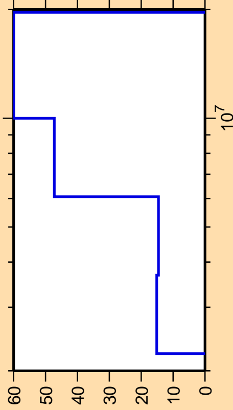
\Delta\sigma/\sigma vs. E for ^{155}\text{Pm}(n,n\text{cont.})
