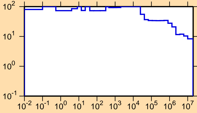
\Delta\sigma/\sigma vs. E for ^{155}\text{Pm}(n,\text{nonel.})
