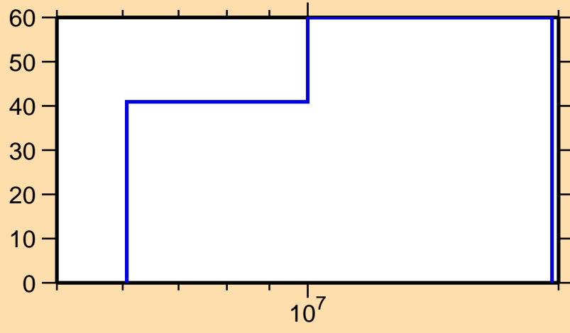
\Delta\sigma/\sigma vs. E for ^{155}\text{Pm}(n,\text{inel.})
