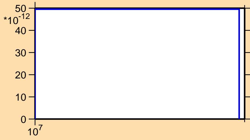
\sigma vs. E for ^{155}\text{Pm}(n,2np)
