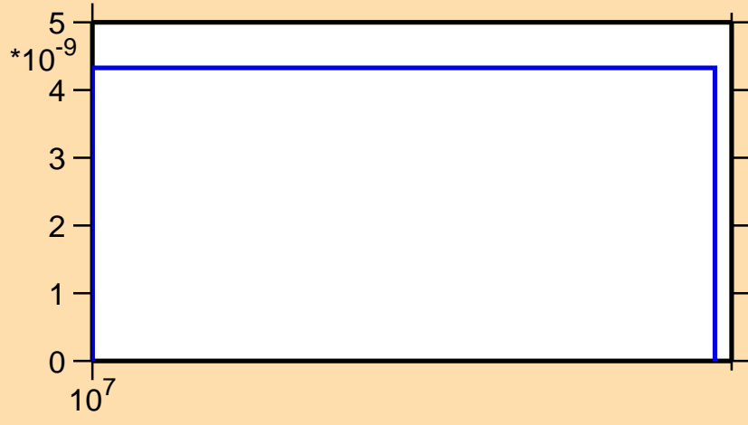
\sigma vs. E for ^{155}\text{Pm}(n,\text{nd})
