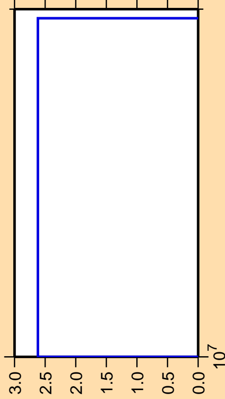
\Delta\sigma/\sigma vs. E for ^{155}\text{Pm}(n,2n\alpha)
