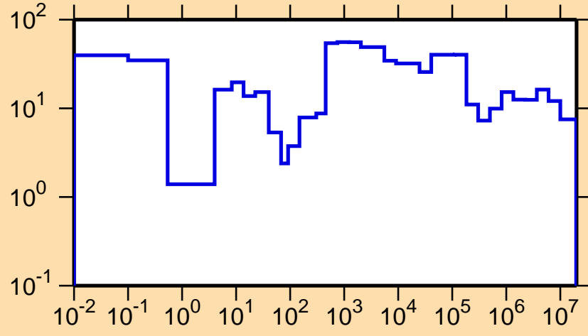
\Delta\sigma/\sigma vs. E for ^{155}\text{Pm}(n,\text{tot.})
