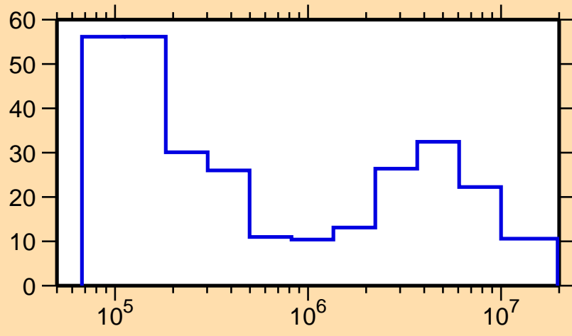
\Delta\sigma/\sigma vs. E for ^{155}\text{Pm}(n,\text{el.})
