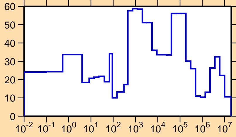
\Delta\sigma/\sigma vs. E for ^{155}\text{Pm}(n,\text{el.})
