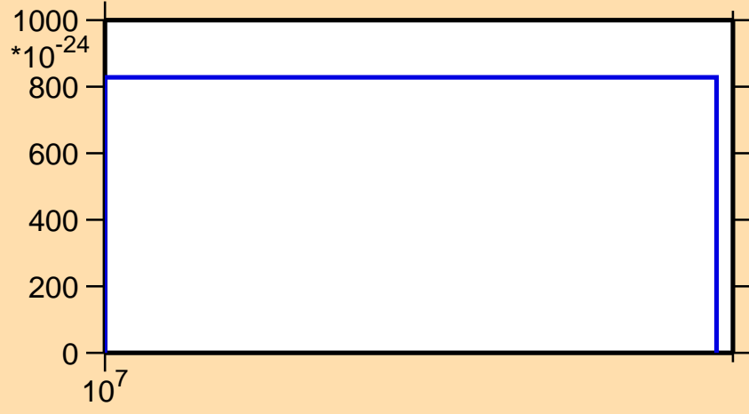
\sigma vs. E for ^{155}\text{Pm} (mt 11)
