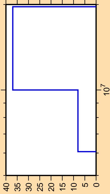
\Delta\sigma/\sigma vs. E for ^{155}\text{Pm}(n,2n)
