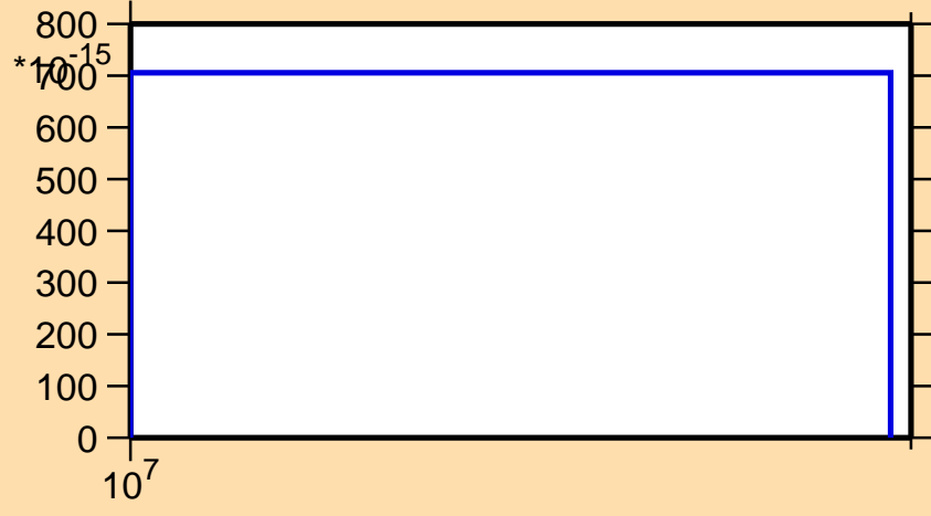
\sigma vs. E for ^{155}\text{Pm}(n,2n\alpha)
