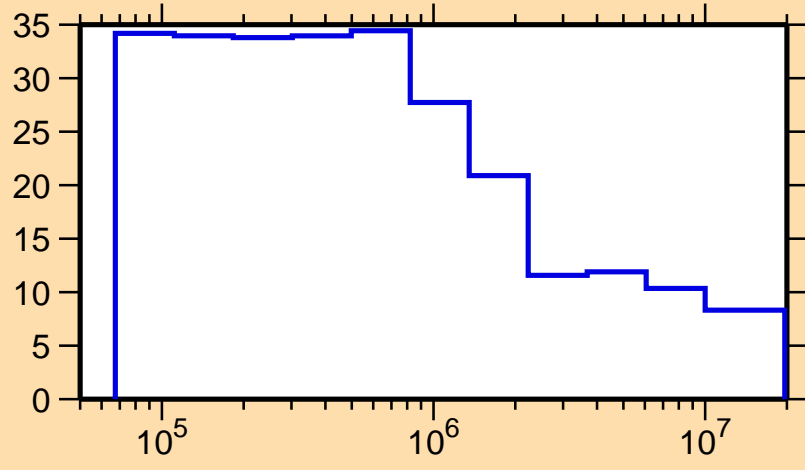
\Delta\sigma/\sigma vs. E for ^{155}\text{Pm}(n,\text{nonel.})
