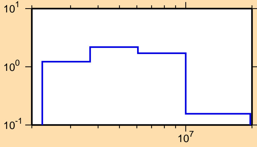
\sigma vs. E for ^{155}\text{Pm}(n,n\text{cont.})
