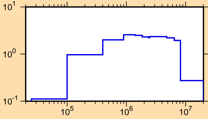
\sigma vs. E for ^{155}\text{Pm}(n,\text{inel.})
