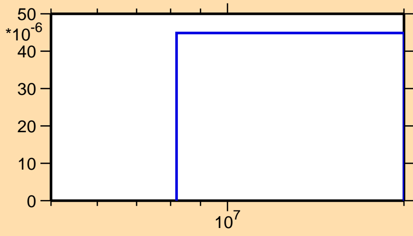
\sigma vs. E for ^{155}\text{Pm}(n,np)
