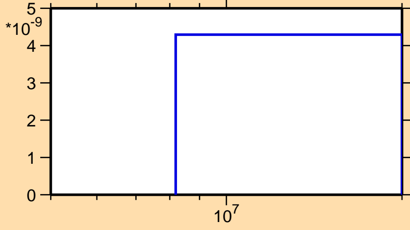
\sigma vs. E for ^{155}\text{Pm}(n,nd)
