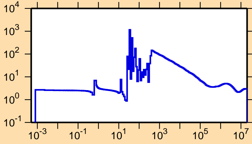
\sigma vs. E for ^{156}\text{Pm}(n,\text{el.})
