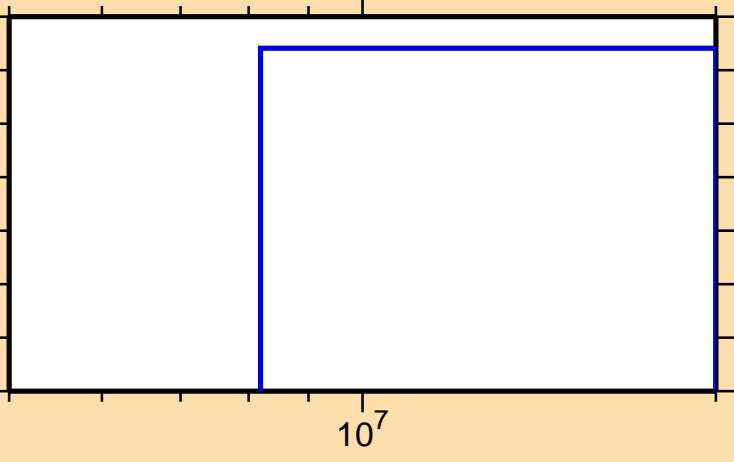
\sigma vs. E for ^{156}\text{Pm}(n,nd)
