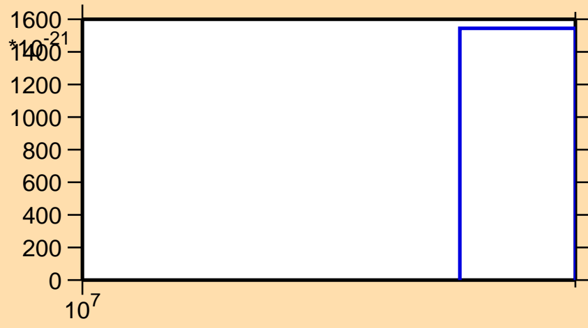
\sigma vs. E for ^{156}\text{Pm} (mt 11)
