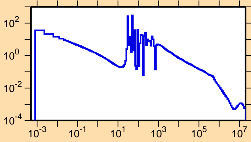
\sigma vs. E for ^{156}\text{Pm}(n,\gamma)
