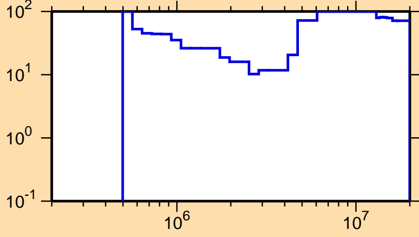
\Delta\sigma/\sigma vs. E for ^{156}\text{Pm}(n,n\text{cont.})
