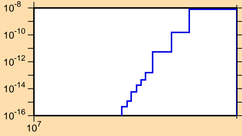
\sigma vs. E for ^{156}\text{Pm}(n,2n\alpha)
