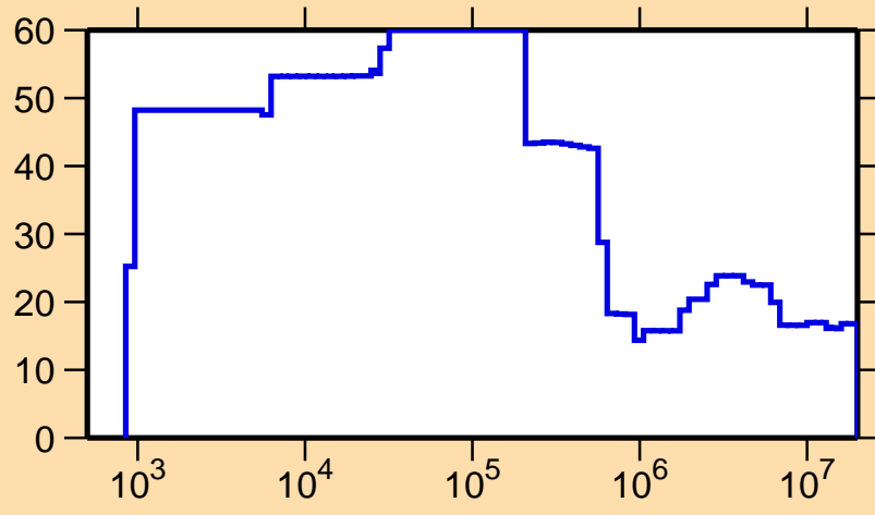
\Delta\sigma/\sigma vs. E for ^{156}\text{Pm}(n,\text{el.})
