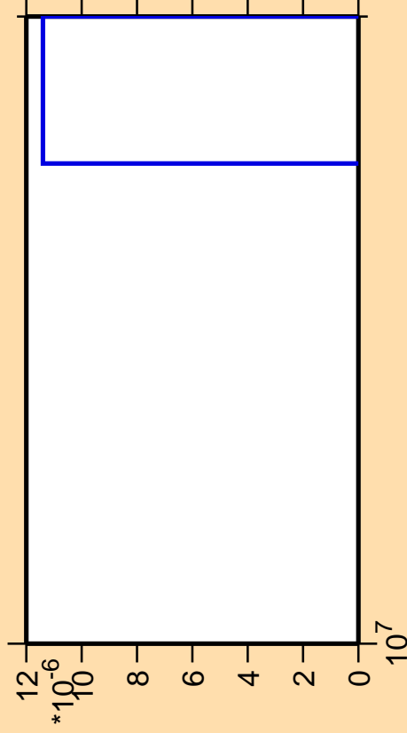
\Delta\sigma/\sigma vs. E for ^{156}\text{Pm} (mt 11)
