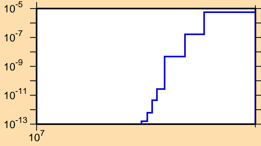
\sigma vs. E for ^{156}\text{Pm}(n,nd)
