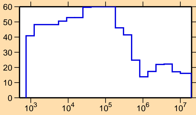
\Delta\sigma/\sigma vs. E for ^{156}\text{Pm}(n,el.)
