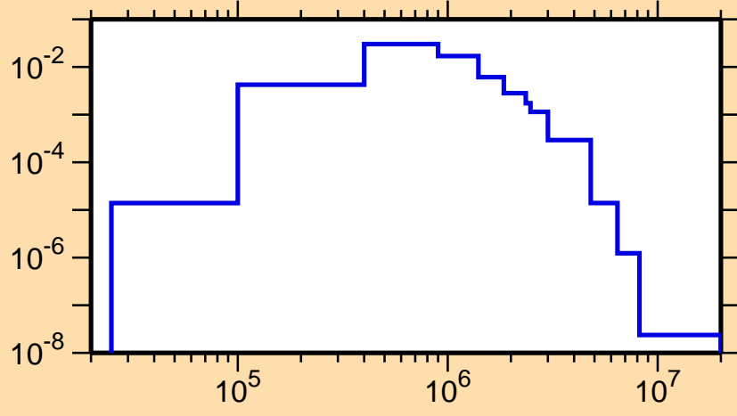
\sigma vs. E for ^{156}\text{Pm}(n,n_4)
