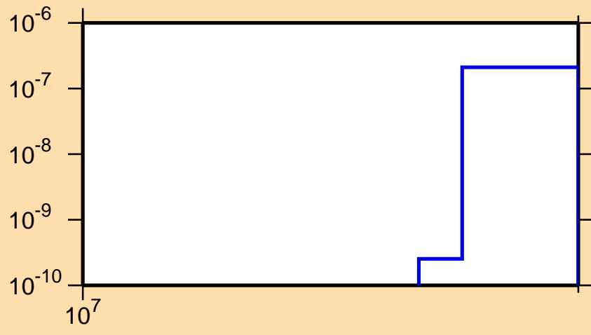
\sigma vs. E for ^{157}\text{Pm}(n,nd)
