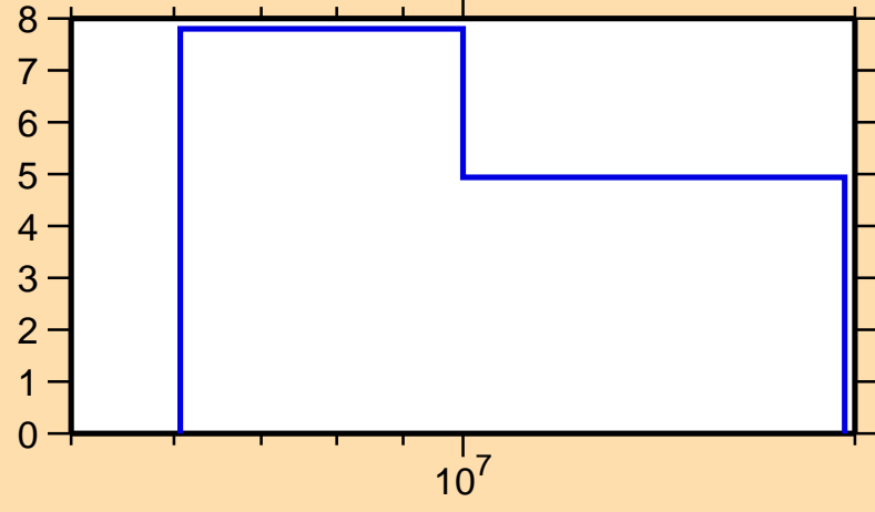
\Delta\sigma/\sigma vs. E for ^{157}\text{Pm}(n,\text{tot.})
