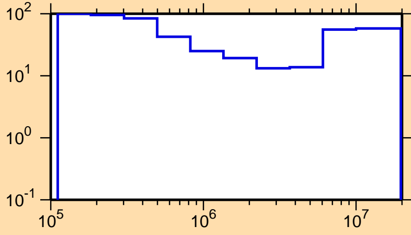
\Delta\sigma/\sigma vs. E for ^{157}\text{Pm}(n,n\text{cont.})
