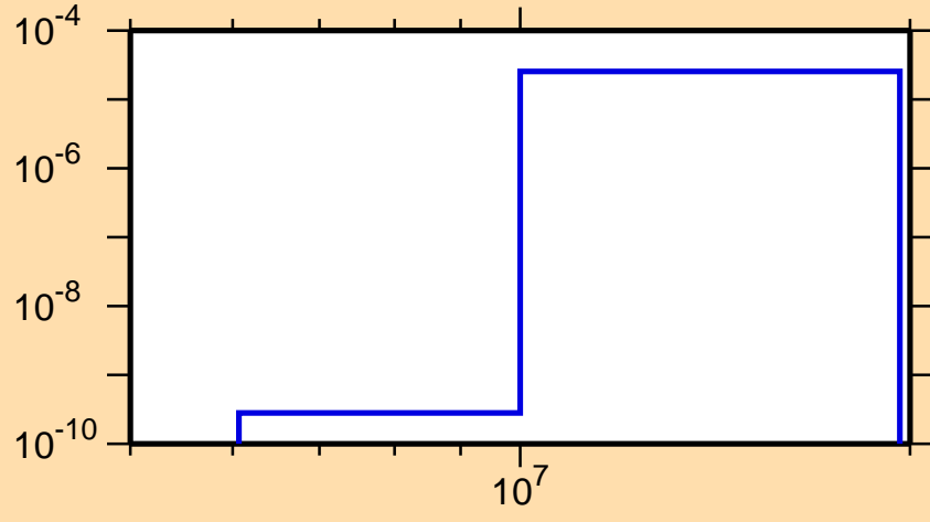
\sigma vs. E for ^{157}\text{Pm}(n,\alpha)
