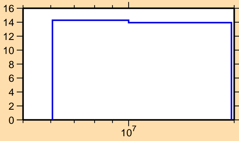
\Delta\sigma/\sigma vs. E for ^{157}\text{Pm}(n,el.)
