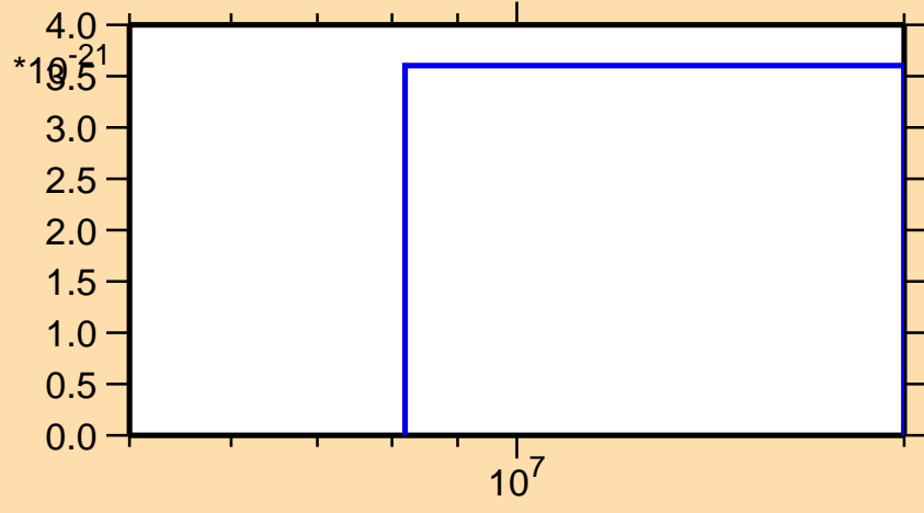
\sigma vs. E for ^{157}\text{Pm} (mt 11)
