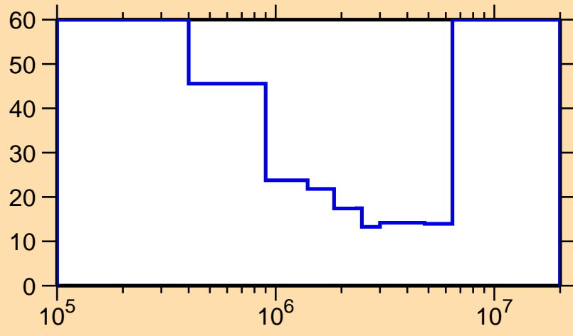
\Delta\sigma/\sigma vs. E for ^{157}\text{Pm}(n,n\text{cont.})
