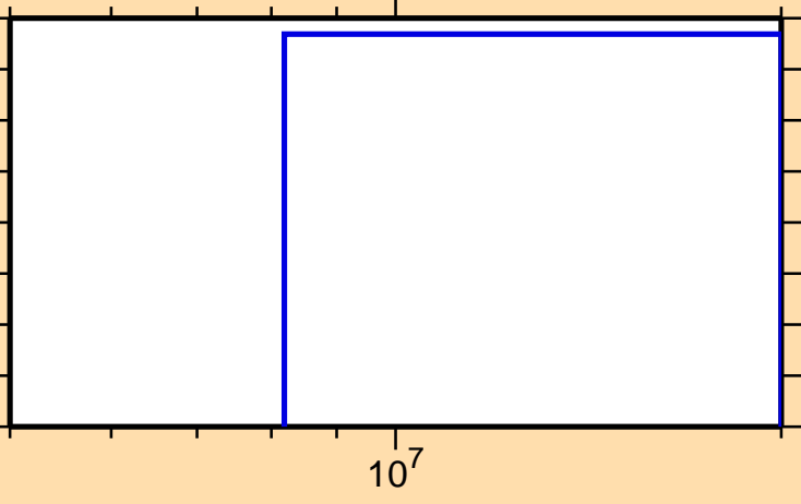
\sigma vs. E for ^{157}\text{Pm}(n,n\alpha)
