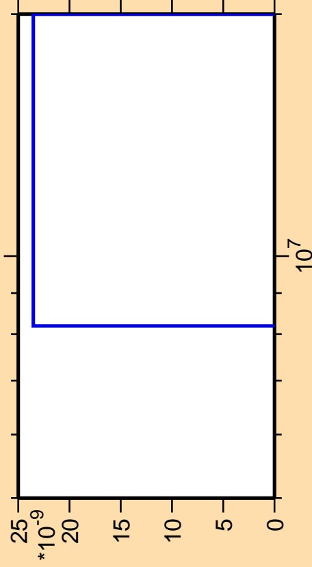
\Delta\sigma/\sigma vs. E for ^{157}\text{Pm} (mt 11)
