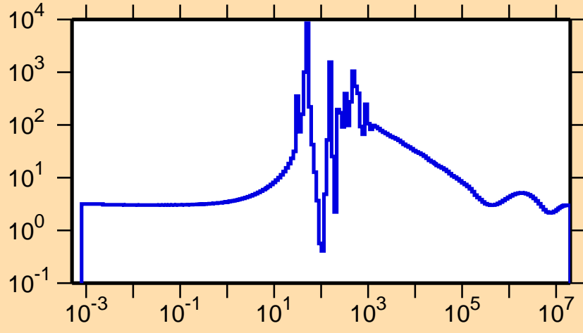
\sigma vs. E for ^{158}\text{Pm}(n,\text{el.})
