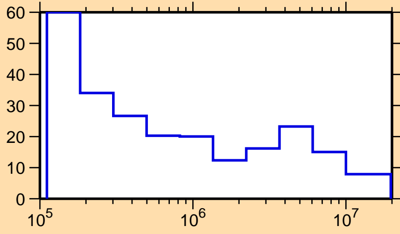
\Delta\sigma/\sigma vs. E for ^{158}\text{Pm}(n,\text{tot.})
