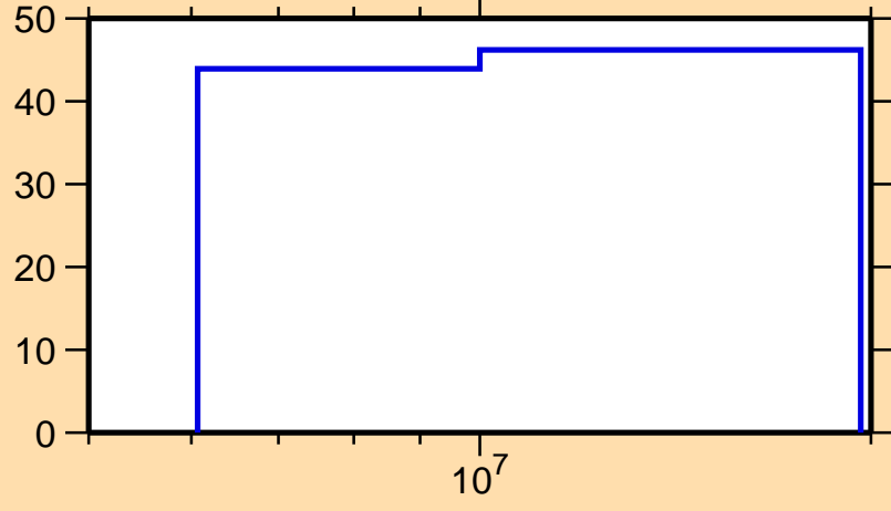
\Delta\sigma/\sigma vs. E for ^{158}\text{Pm}(n,\gamma)
