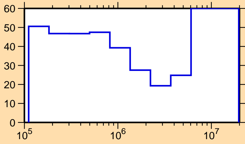
\Delta\sigma/\sigma vs. E for ^{158}\text{Pm}(n,\text{inel.})
