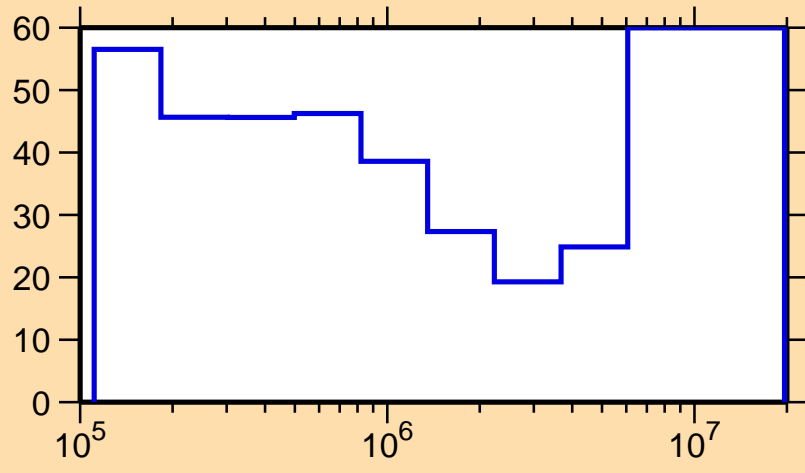
\Delta\sigma/\sigma vs. E for ^{158}\text{Pm}(n,n\text{cont.})
