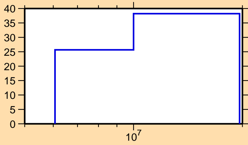
\Delta\sigma/\sigma vs. E for ^{158}\text{Pm}(n,2n)
