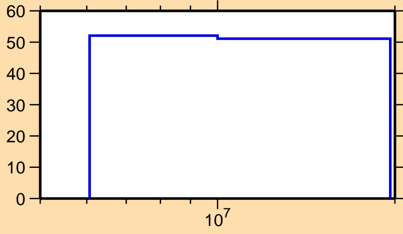
\Delta\sigma/\sigma vs. E for ^{158}\text{Pm}(n,p)
