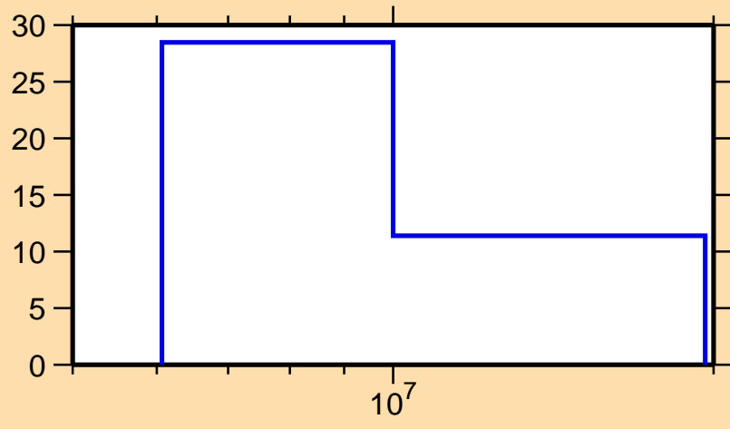
\Delta\sigma/\sigma vs. E for ^{158}\text{Pm}(n,el.)
