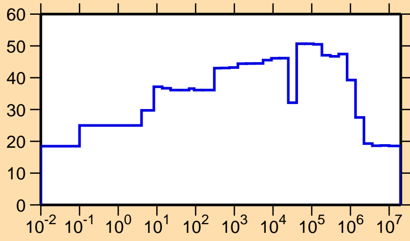
\Delta\sigma/\sigma vs. E for ^{158}\text{Pm}(n,\text{nonel.})
