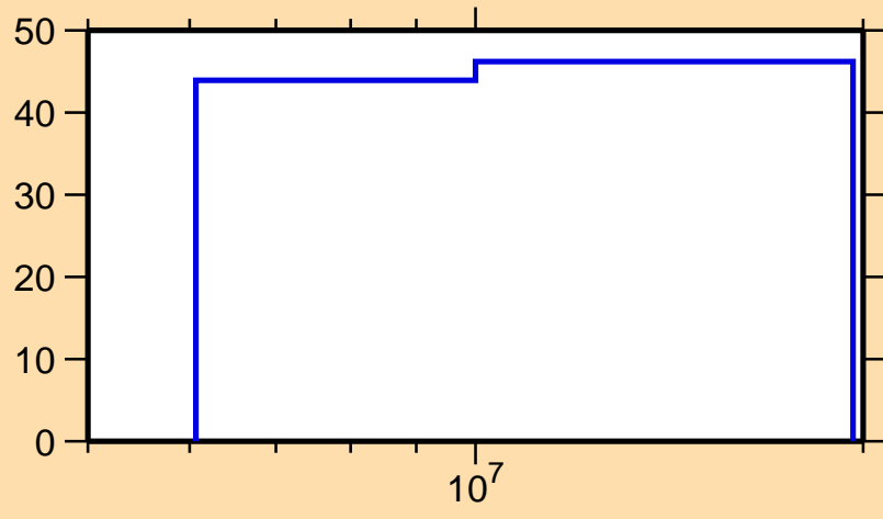
\Delta\sigma/\sigma vs. E for ^{158}\text{Pm}(n,\gamma)
