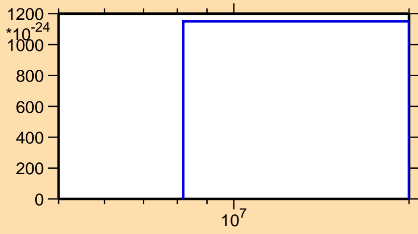
\sigma vs. E for ^{158}\text{Pm}(\text{mt } 11)
