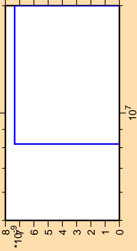
\Delta\sigma/\sigma vs. E for ^{158}\text{Pm}(\text{mt } 11)
