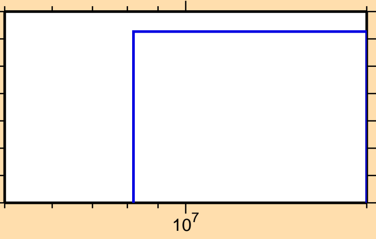
\sigma vs. E for ^{159}\text{Pm}(n,2np)
