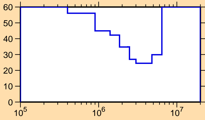
\Delta\sigma/\sigma vs. E for ^{159}\text{Pm}(n,n\text{cont.})
