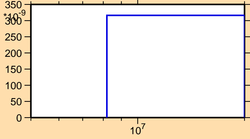
\sigma vs. E for ^{159}\text{Pm}(n,n\alpha)
