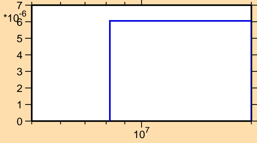
\sigma vs. E for ^{159}\text{Pm}(n,t)
