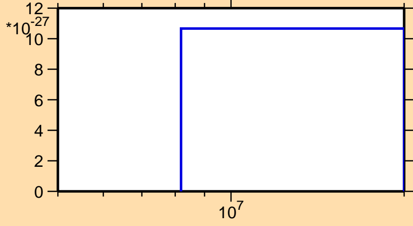
\sigma vs. E for ^{159}\text{Pm} (mt 42)
