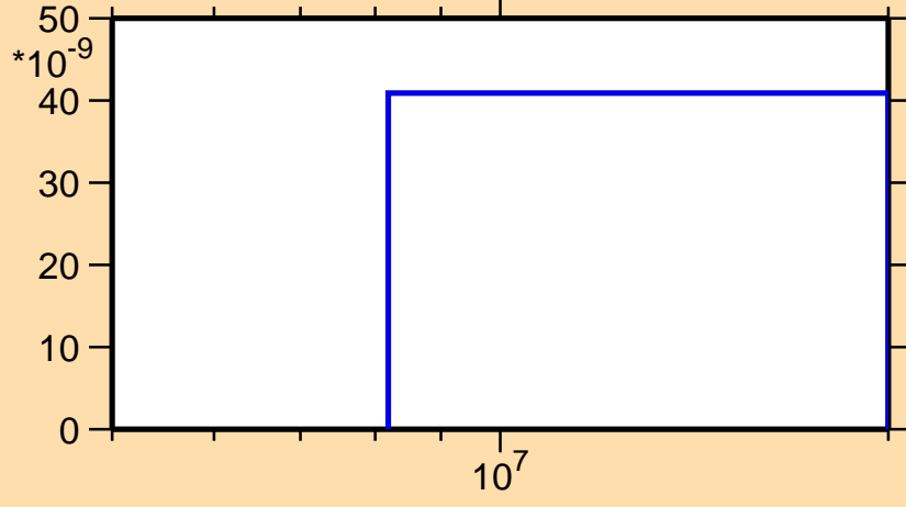
\sigma vs. E for ^{159}\text{Pm}(n,nt)
