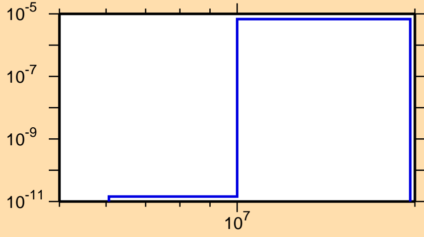
\sigma vs. E for ^{160}\text{Pm}(n,\alpha)
