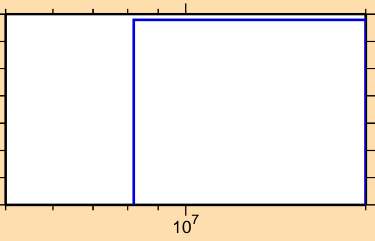
\sigma vs. E for ^{160}\text{Pm}(n,np)
