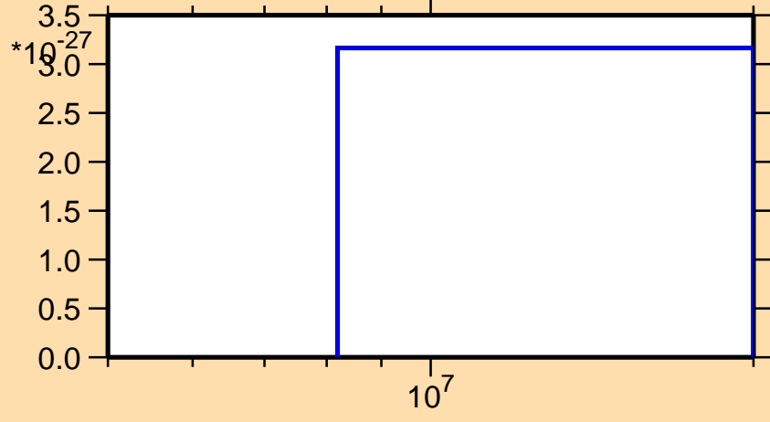
\sigma vs. E for ^{160}\text{Pm} (mt 42)
