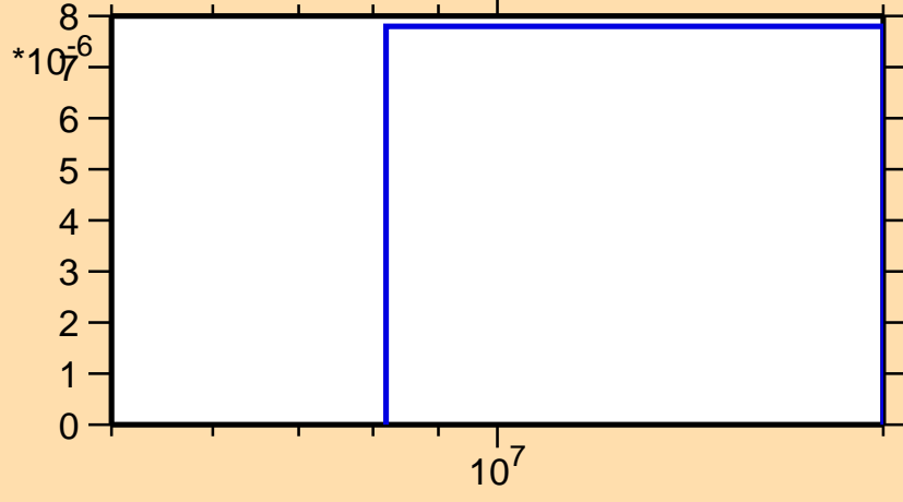
\sigma vs. E for ^{160}\text{Pm}(n,t)
