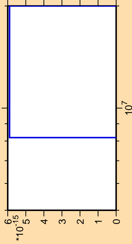
\Delta\sigma/\sigma vs. E for ^{160}\text{Pm} (mt 42)
