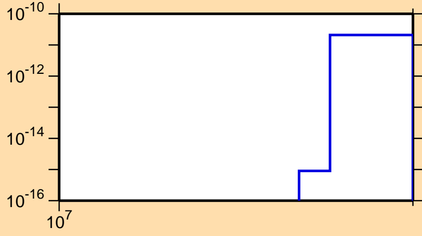
\sigma vs. E for ^{195}\text{Po}(n,nt)
