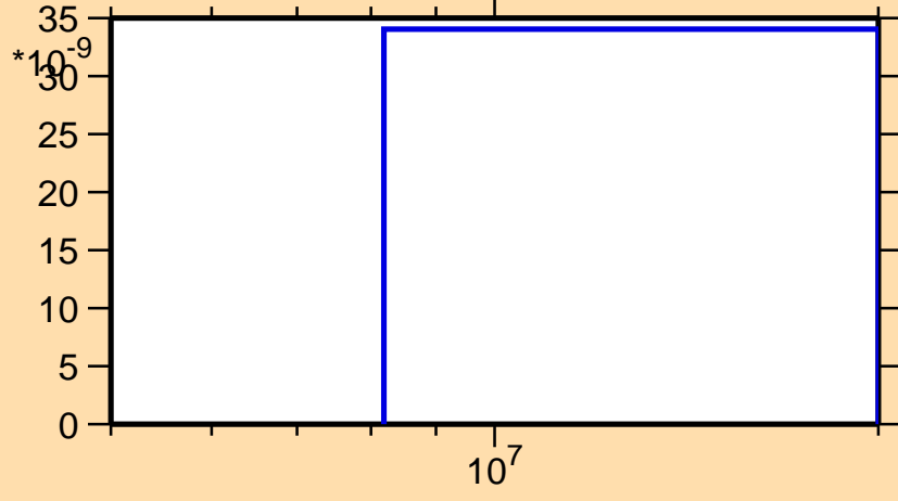
\sigma vs. E for ^{195}\text{Po}(n,\text{nd})
