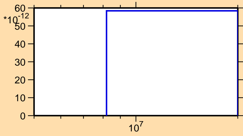
\sigma vs. E for ^{195}\text{Po}(\text{mt } 34)
