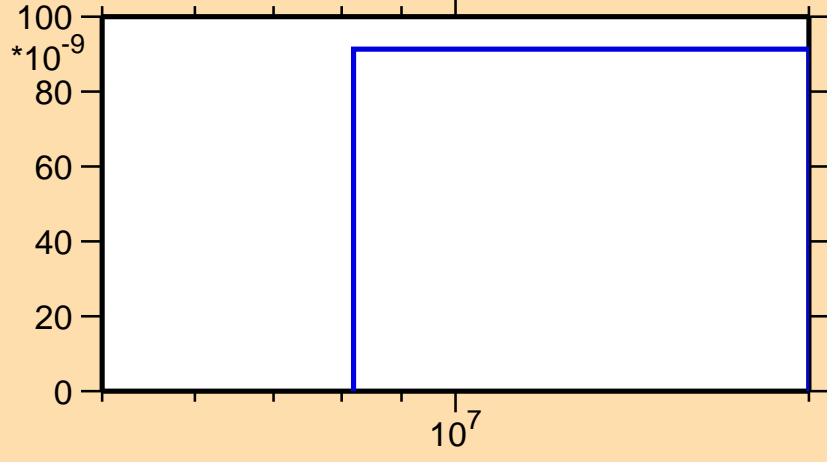
\sigma vs. E for ^{195}\text{Po}(n,\text{pd})
