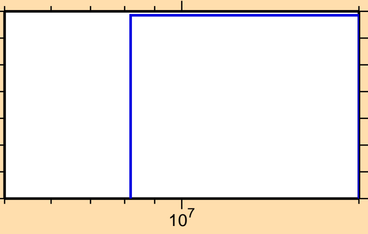
\sigma vs. E for ^{195}\text{Po}(\text{mt } 45)
