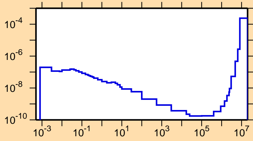
\sigma vs. E for ^{195}\text{Po}(n,p\alpha)
