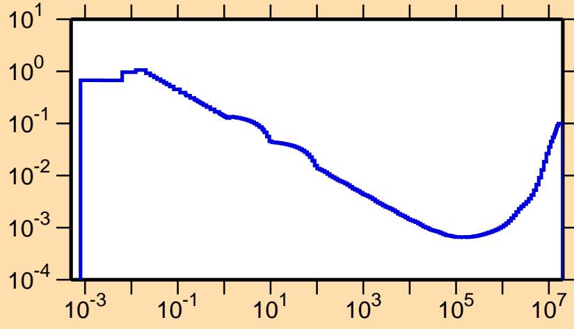
\sigma vs. E for ^{195}\text{Po}(n,\alpha)
