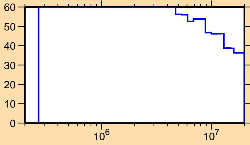
\Delta\sigma/\sigma vs. E for ^{195}\text{Po}(n,n\text{cont.})
