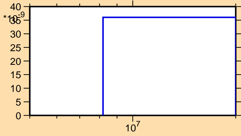
\sigma vs. E for ^{195}\text{Po}(\text{mt } 45)
