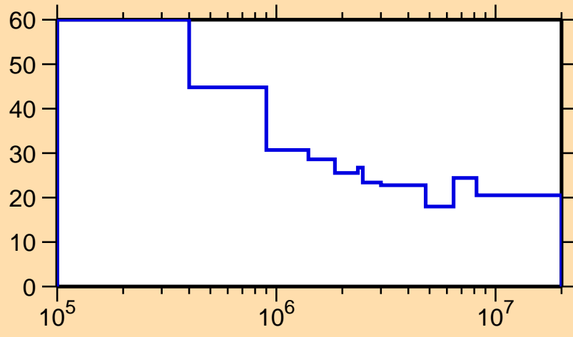
\Delta\sigma/\sigma vs. E for ^{195}\text{Po}(n, n_1)
