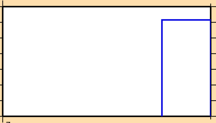
\sigma vs. E for ^{196}\text{Po}(n,3n)
