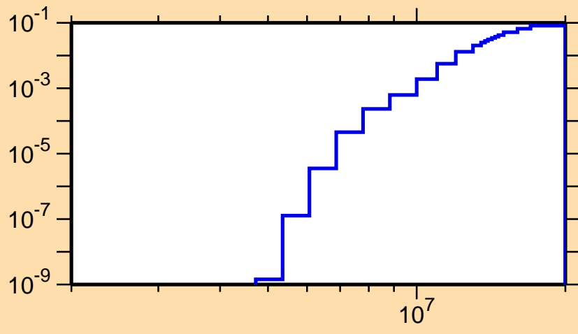
\sigma vs. E for ^{196}\text{Po}(n,np)
