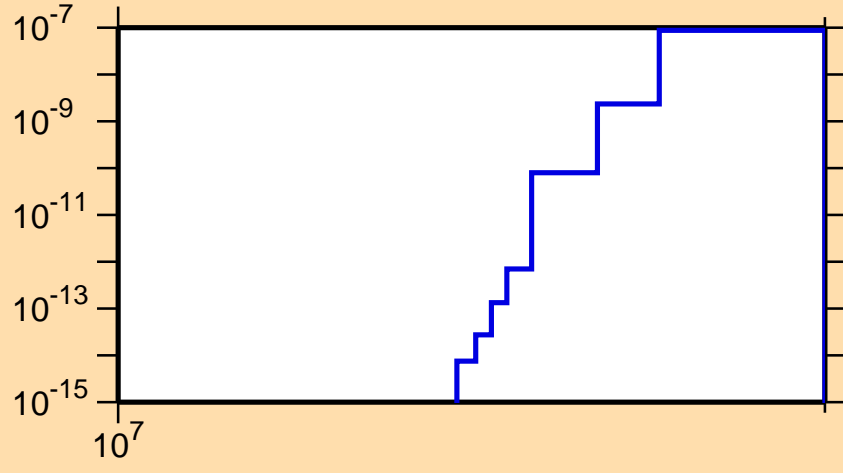
\sigma vs. E for ^{196}\text{Po}(n,\text{nd})
