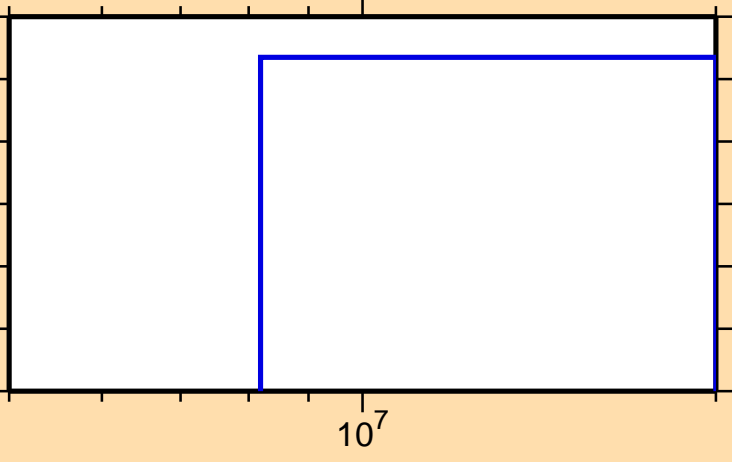
\sigma vs. E for ^{196}\text{Po}(n,t)
