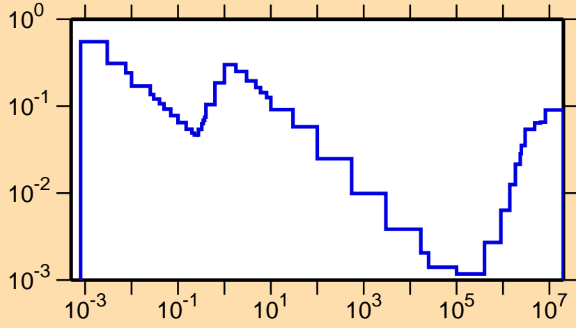
\sigma vs. E for ^{196}\text{Po}(n,p)
