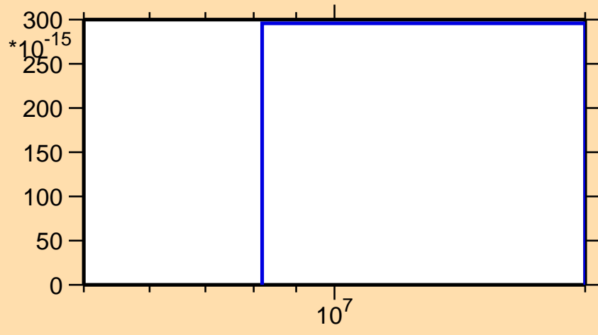
\sigma vs. E for ^{196}\text{Po}(n,nt)
