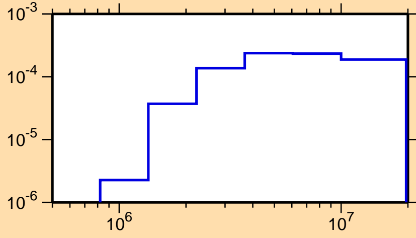
\sigma vs. E for ^{197}\text{Po}(n,n_3)
