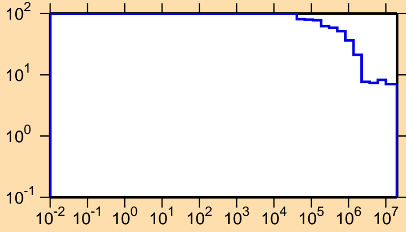
\Delta\sigma/\sigma vs. E for ^{197}\text{Po}(n,\text{nonel.})
