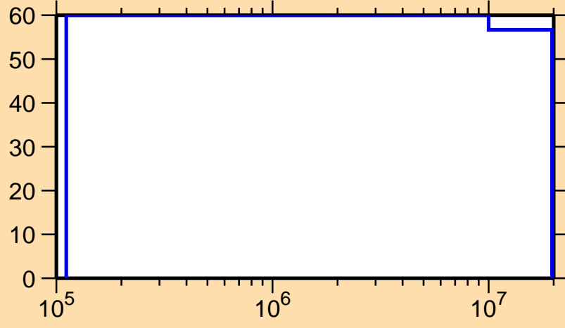
\Delta\sigma/\sigma vs. E for ^{197}\text{Po}(n,n_1)
