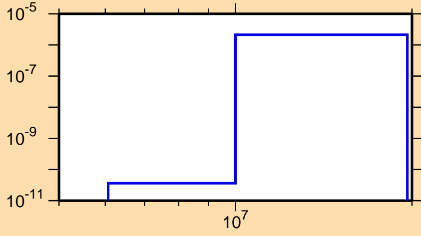
\sigma vs. E for ^{197}\text{Po}(n,\text{He}3)
