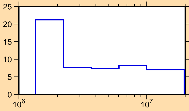
\Delta\sigma/\sigma vs. E for ^{197}\text{Po}(n,\text{nonel.})
