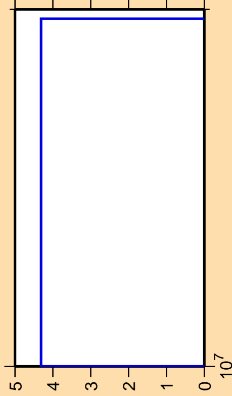
\Delta\sigma/\sigma vs. E for ^{197}\text{Po}(n,nt)
