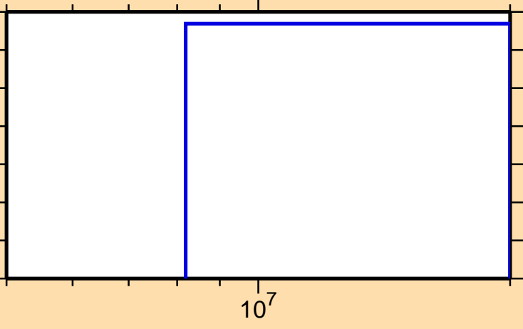
\sigma vs. E for ^{197}\text{Po}(n,3n)
