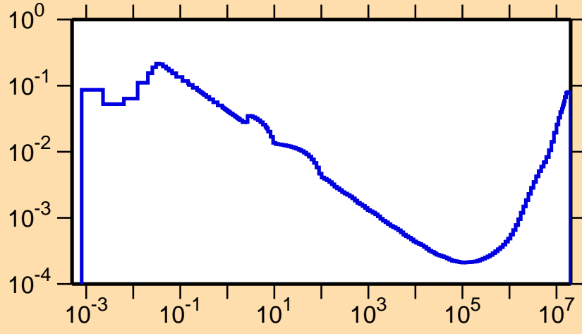
\sigma vs. E for ^{197}\text{Po}(n,\alpha)
