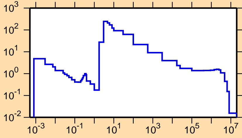
\sigma vs. E for ^{197}\text{Po}(n,\gamma)
