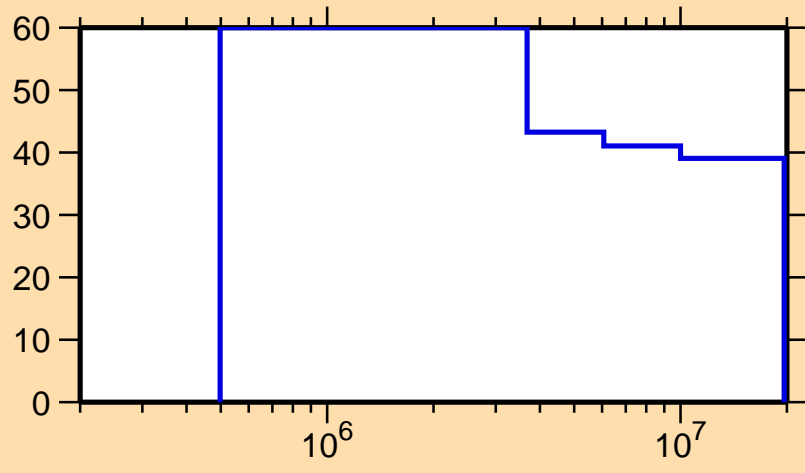
\Delta\sigma/\sigma vs. E for ^{198}\text{Po}(n,n_1)
