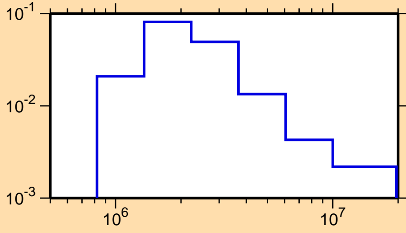
\sigma vs. E for ^{198}\text{Po}(n,n_3)
