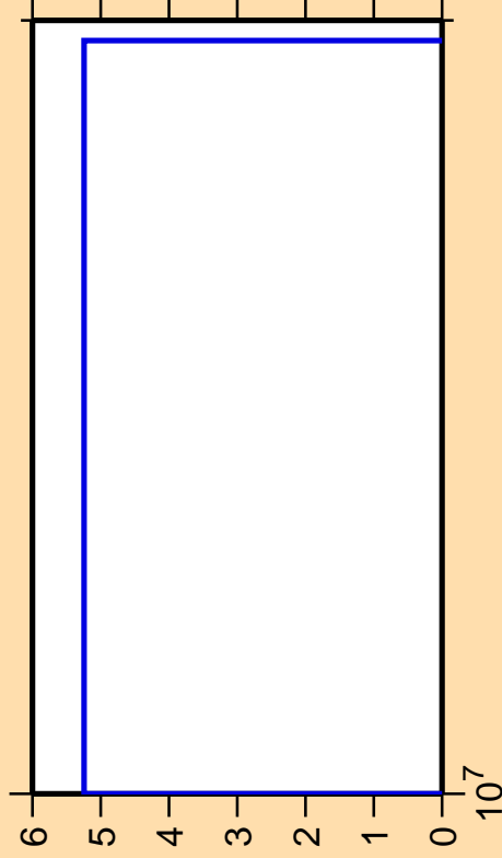
\Delta\sigma/\sigma vs. E for ^{198}\text{Po}(n,nt)
