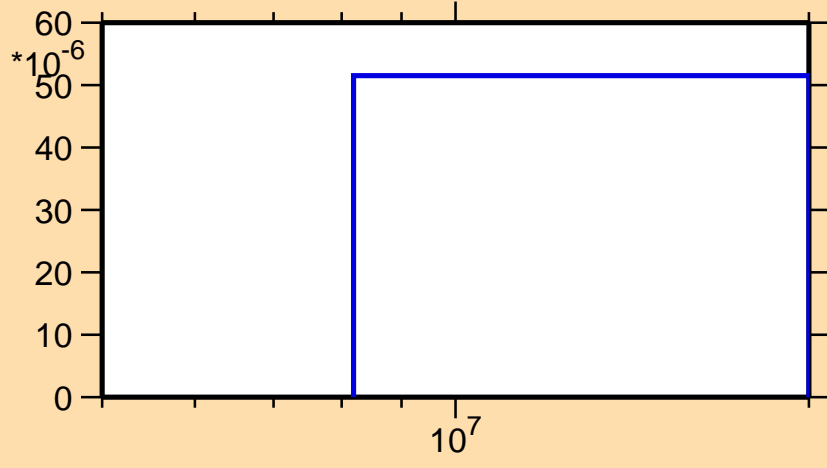
\sigma vs. E for ^{198}\text{Po}(n,t)
