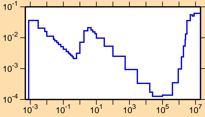
\sigma vs. E for ^{198}\text{Po}(n,p)
