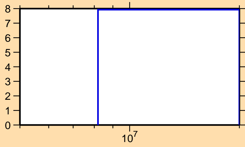
\Delta\sigma/\sigma vs. E for ^{198}\text{Po}(n,\text{el.})
