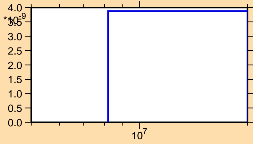
\sigma vs. E for ^{198}\text{Po}(\text{mt } 45)
