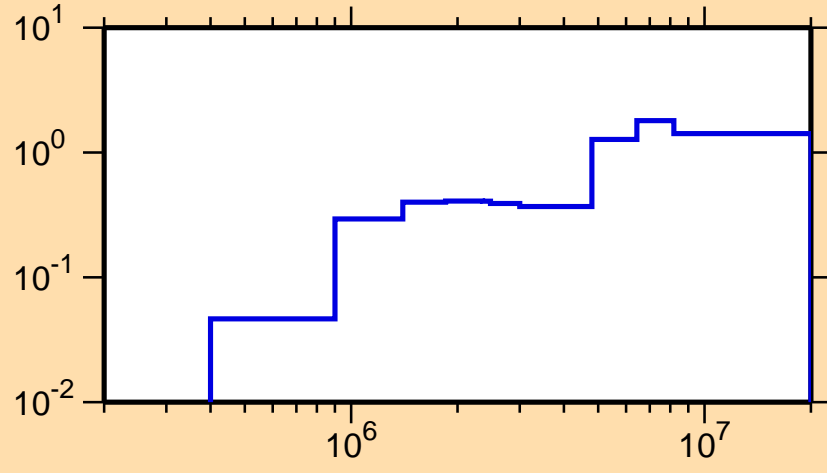
\sigma vs. E for ^{198}\text{Po}(n,\text{inel.})
