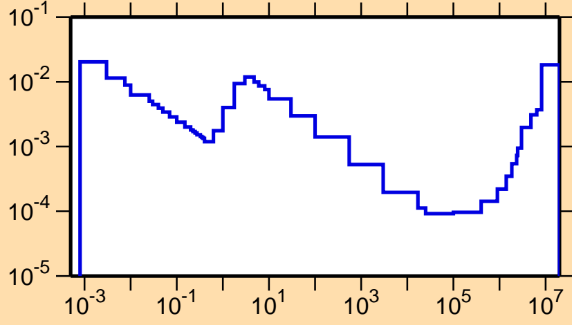
\sigma vs. E for ^{198}\text{Po}(n,\alpha)
