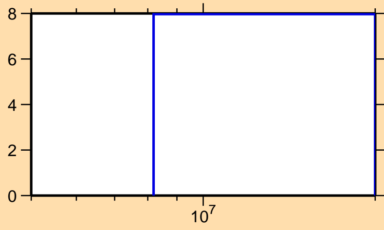
\Delta\sigma/\sigma vs. E for ^{198}\text{Po}(n,\text{nonel.})
