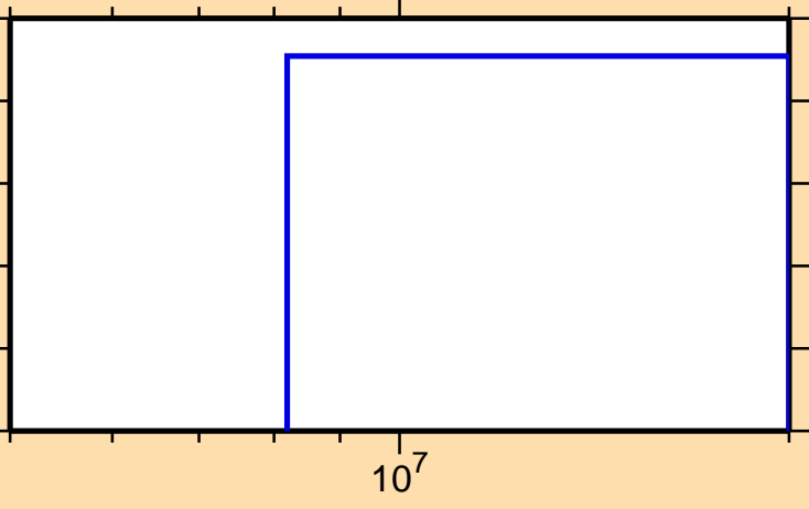
\sigma vs. E for ^{199}\text{Po}(n,\text{nd})
