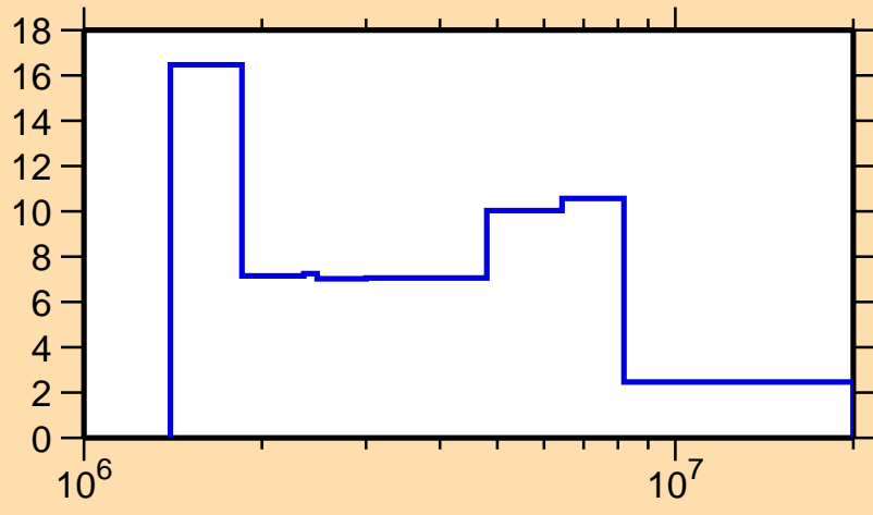
\Delta\sigma/\sigma vs. E for ^{199}\text{Po}(n,\text{tot.})
