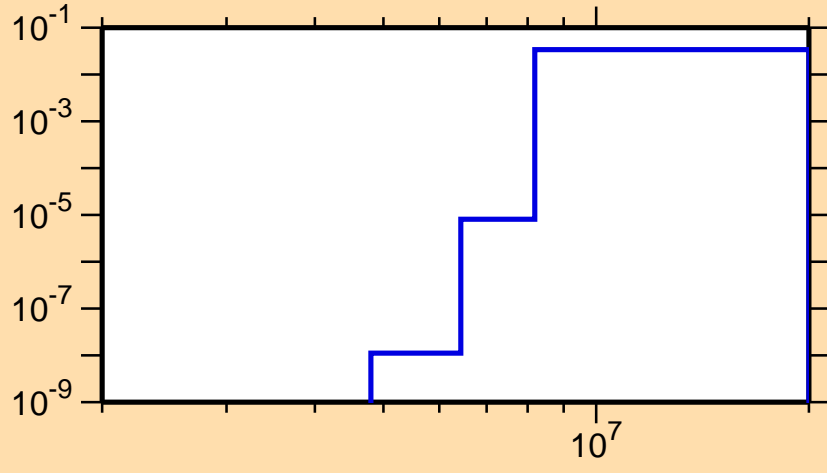
\sigma vs. E for ^{199}\text{Po}(n,np)
