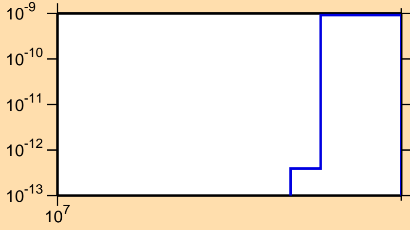
\sigma vs. E for ^{199}\text{Po}(n,nt)
