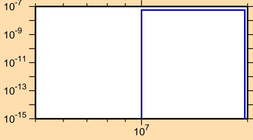
\sigma vs. E for ^{199}\text{Po}(n,nd)
