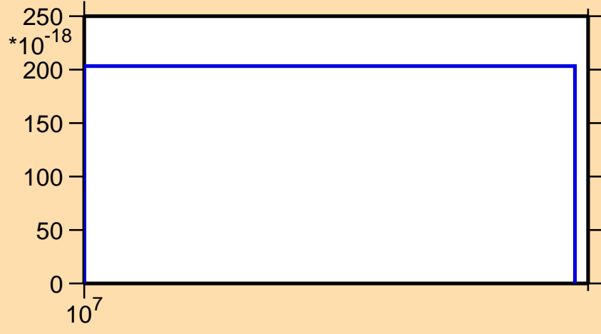
\sigma vs. E for ^{199}\text{Po}(n,3n\alpha)
