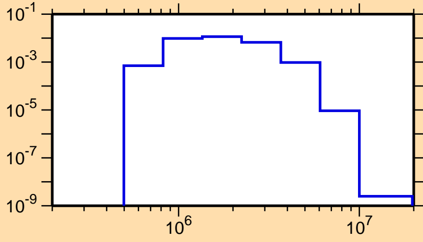
\sigma vs. E for ^{199}\text{Po}(n,n_4)
