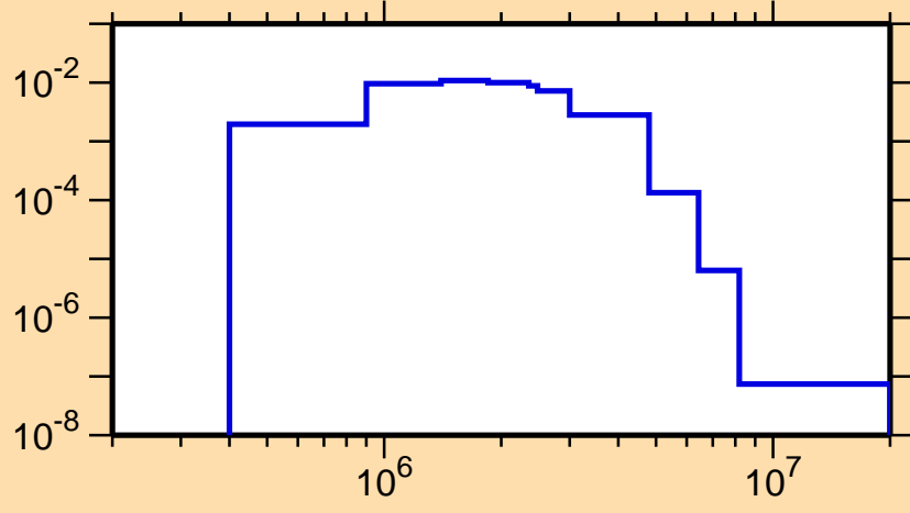
\sigma vs. E for ^{199}\text{Po}(n,n_3)
