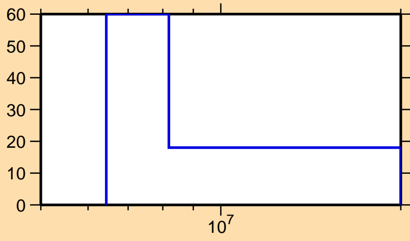
\Delta\sigma/\sigma vs. E for ^{199}\text{Po}(n,2n)
