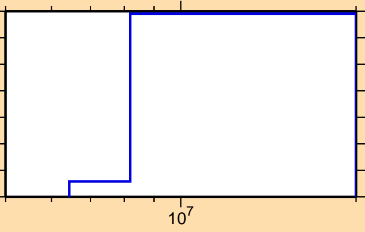
\sigma vs. E for ^{199}\text{Po}(n,\text{He}3)
