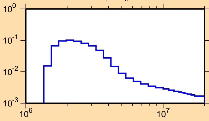
\sigma vs. E for ^{200}\text{Po}(n,n_4)
