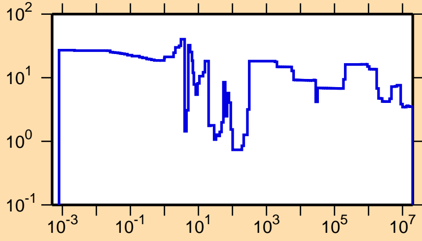
\Delta\sigma/\sigma vs. E for ^{200}\text{Po}(n,\text{tot.})
