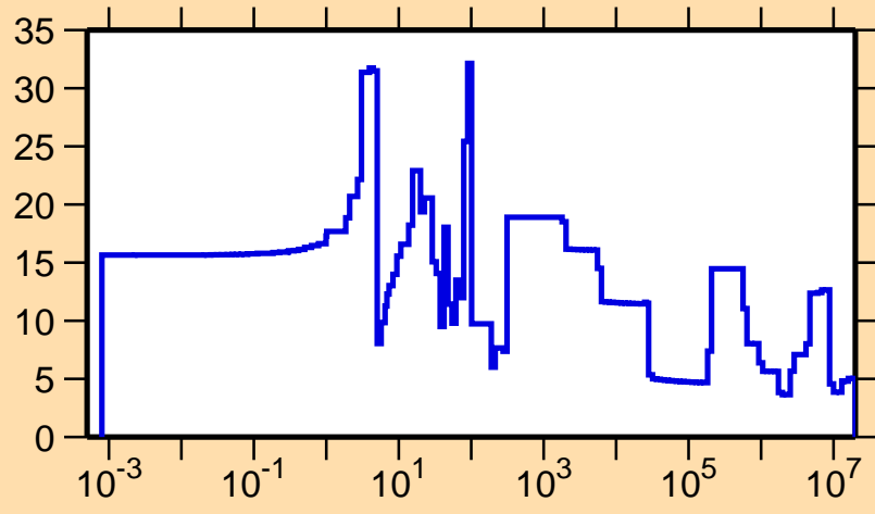
\Delta\sigma/\sigma vs. E for ^{200}\text{Po}(n,\text{el.})
