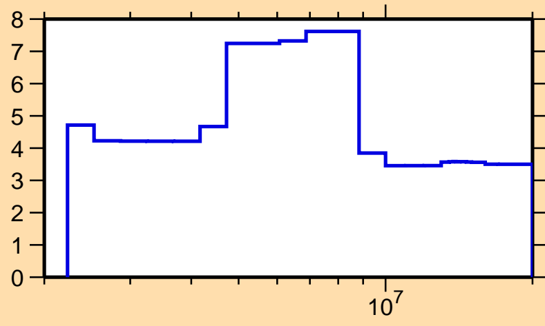
\Delta\sigma/\sigma vs. E for ^{200}\text{Po}(n,\text{tot.})
