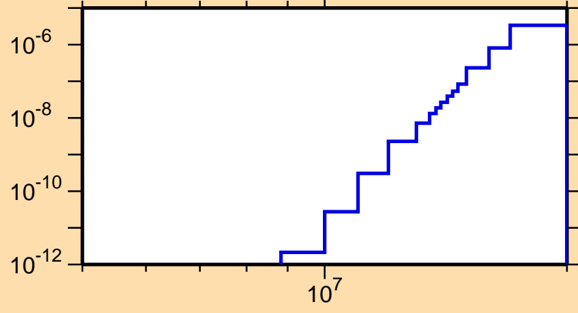
\sigma vs. E for ^{200}\text{Po}(n,\text{He}3)
