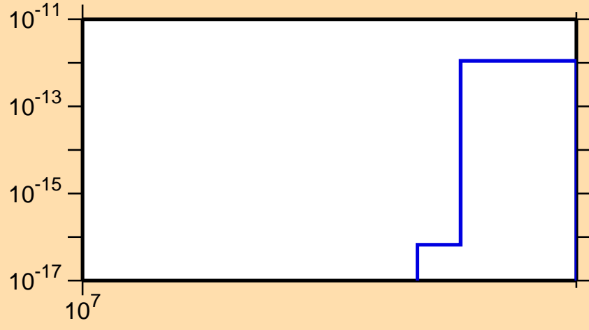
\sigma vs. E for ^{200}\text{Po}(n,3n\alpha)
