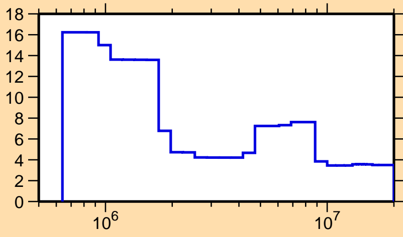
\Delta\sigma/\sigma vs. E for ^{200}\text{Po}(n,\text{tot.})
