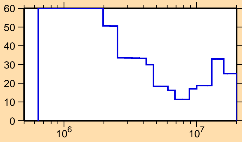
\Delta\sigma/\sigma vs. E for ^{200}\text{Po}(n,\text{inel.})
