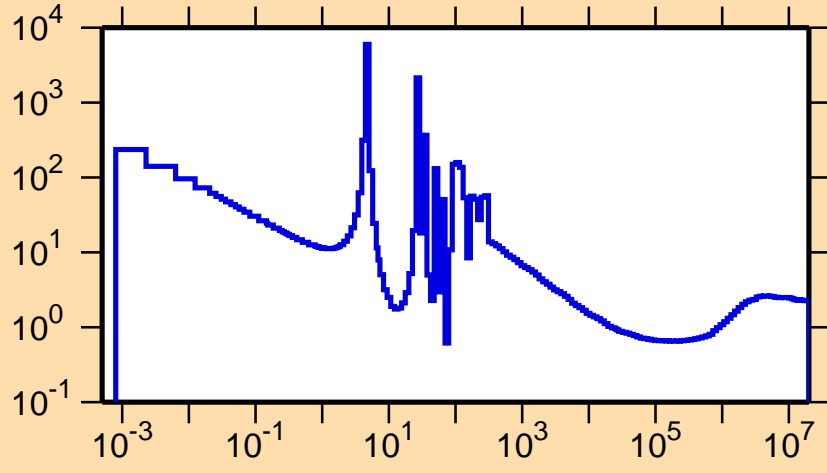
\sigma vs. E for ^{200}\text{Po}(n,\text{nonel.})
