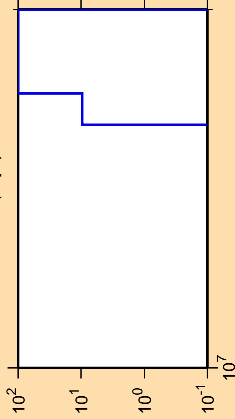
\Delta\sigma/\sigma vs. E for ^{200}\text{Po}(n,\text{pt})
