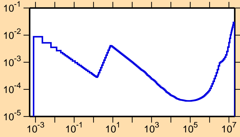
\sigma vs. E for ^{200}\text{Po}(n,\alpha)
