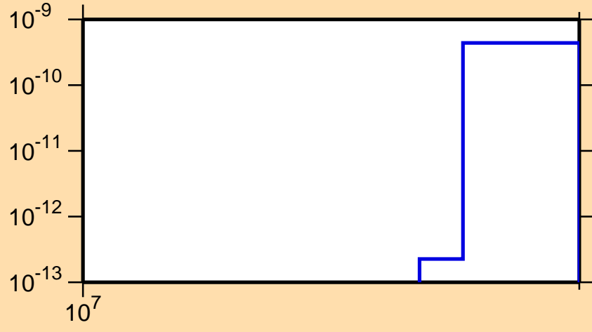
\sigma vs. E for ^{200}\text{Po}(n,nt)
