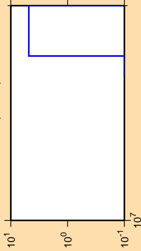
\Delta\sigma/\sigma vs. E for ^{200}\text{Po}(n,3n\alpha)
