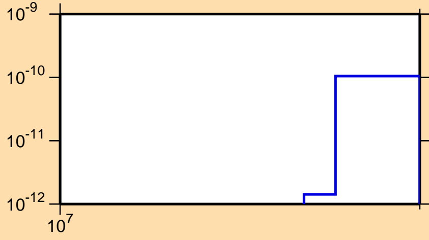
\sigma vs. E for ^{200}\text{Po}(n,\text{pt})
