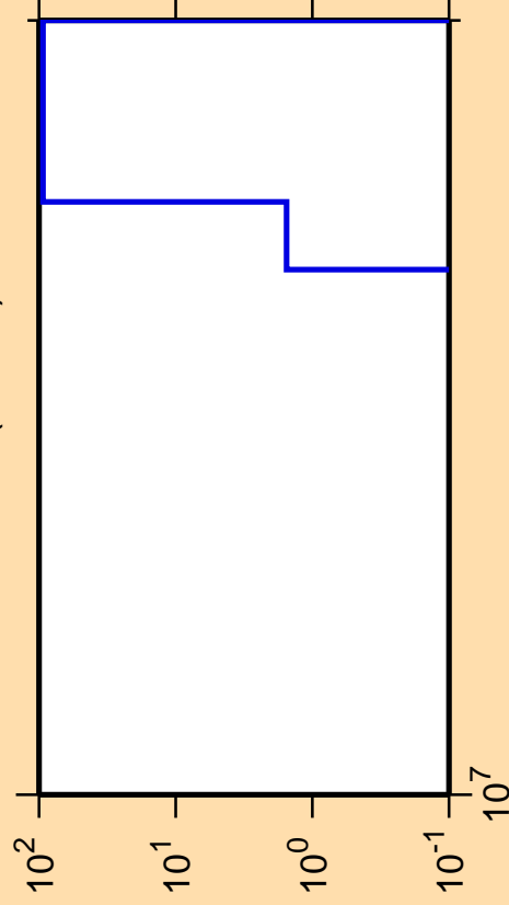
\Delta\sigma/\sigma vs. E for ^{200}\text{Po}(\text{mt } 34)
