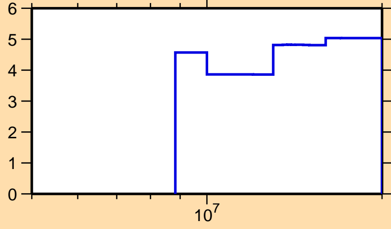
\Delta\sigma/\sigma vs. E for ^{200}\text{Po}(n,\text{el.})
