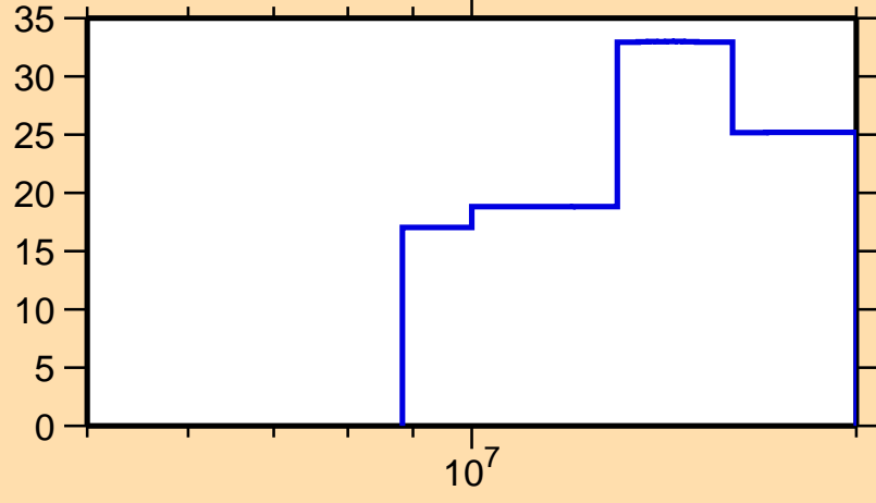
\Delta\sigma/\sigma vs. E for ^{200}\text{Po}(n,\text{inel.})
