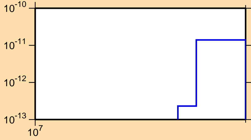
\sigma vs. E for ^{200}\text{Po}(\text{mt } 34)
