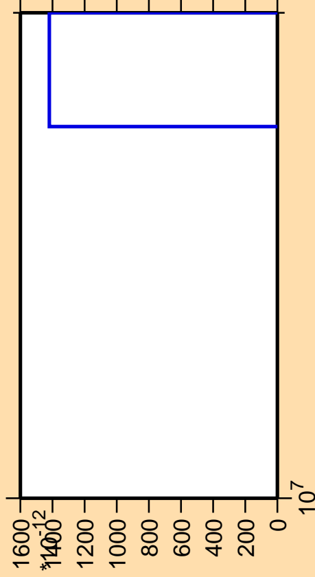
\Delta\sigma/\sigma vs. E for ^{200}\text{Po} (mt 11)
