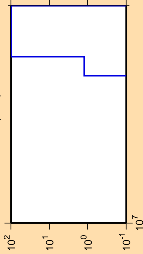
\Delta\sigma/\sigma vs. E for ^{200}\text{Po}(n,nt)
