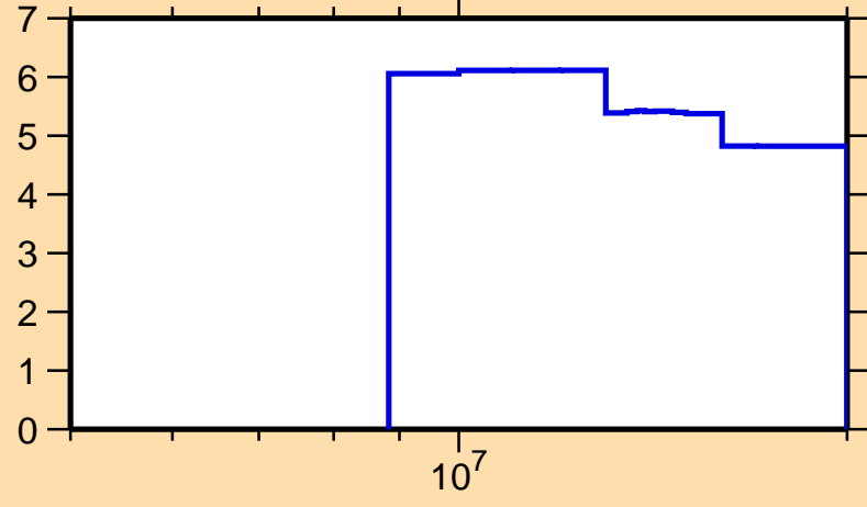
\Delta\sigma/\sigma vs. E for ^{200}\text{Po}(n,\text{nonel.})
