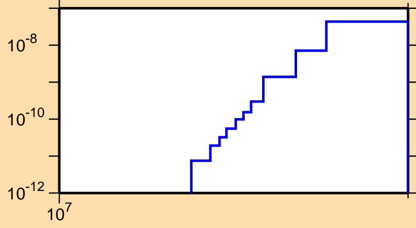
\sigma vs. E for ^{200}\text{Po}(n,\text{pd})
