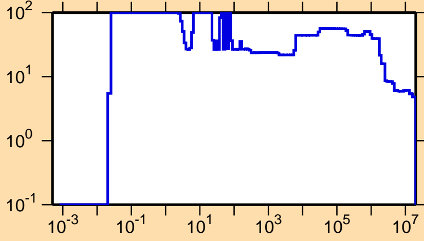
\Delta\sigma/\sigma vs. E for ^{200}\text{Po}(n,\text{nonel.})
