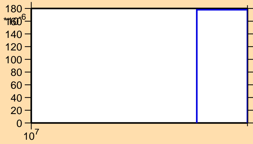
\sigma vs. E for ^{200}\text{Po}(n,3n)
