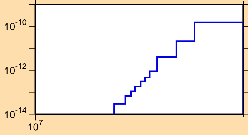
\sigma vs. E for ^{200}\text{Po}(\text{mt117})
