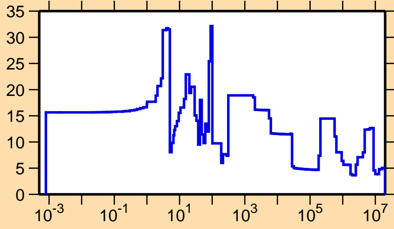
\Delta\sigma/\sigma vs. E for ^{200}\text{Po}(n,\text{el.})
