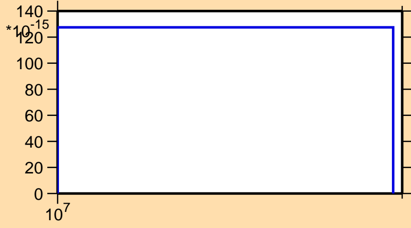
\sigma vs. E for ^{200}\text{Po} (mt 34)
