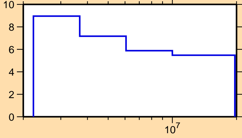
\Delta\sigma/\sigma vs. E for ^{200}\text{Po}(n,n\text{onel.})
