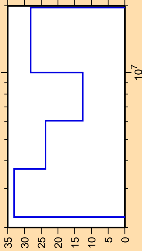
\Delta\sigma/\sigma vs. E for ^{200}\text{Po}(n,n\text{cont.})
