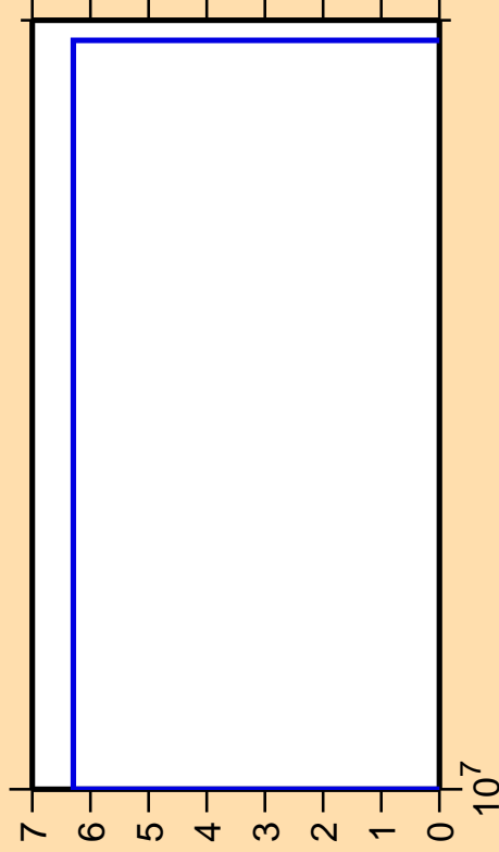
\Delta\sigma/\sigma vs. E for ^{200}\text{Po}(n,\text{pt})
