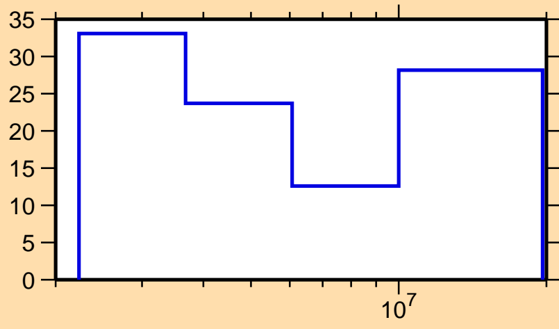
\Delta\sigma/\sigma vs. E for ^{200}\text{Po}(n,n\text{cont.})
