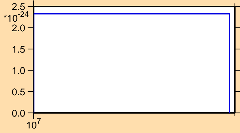
\sigma vs. E for ^{200}\text{Po} (mt 11)
