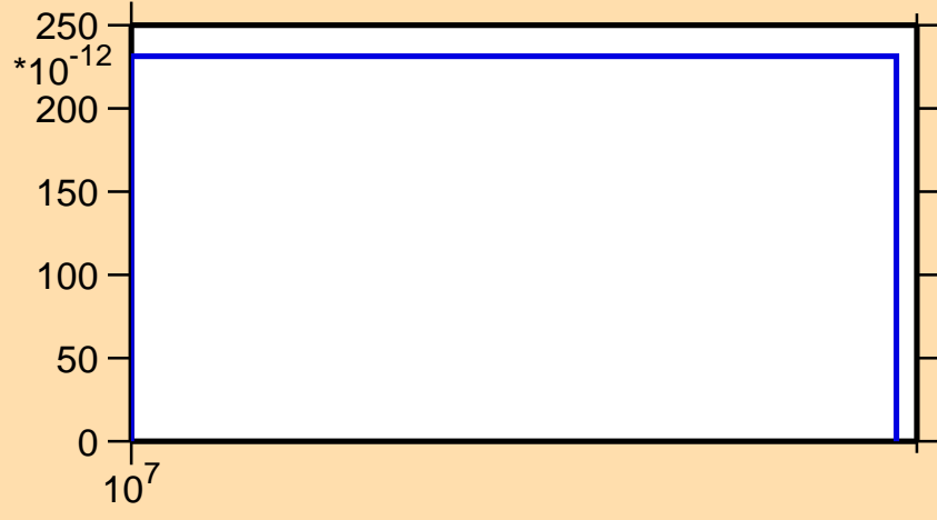
\sigma vs. E for ^{200}\text{Po}(\text{mt } 45)
