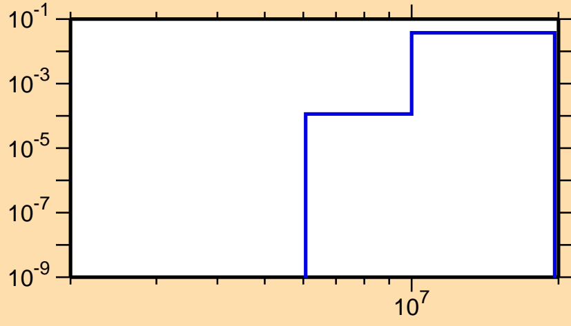
\sigma vs. E for ^{200}\text{Po}(n,np)
