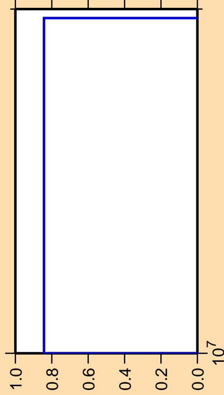
\Delta\sigma/\sigma vs. E for ^{200}\text{Po} (mt 34)
