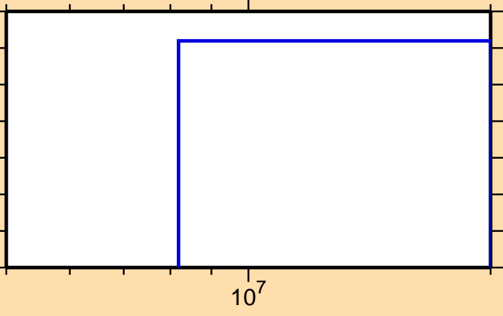
\sigma vs. E for ^{200}\text{Po}(\text{mt } 34)
