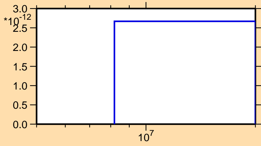
\sigma vs. E for ^{200}\text{Po}(\text{mt117})
