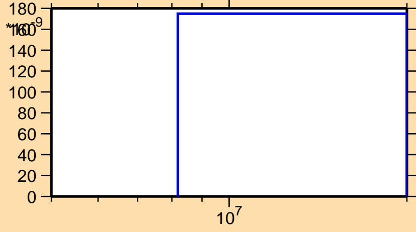
\sigma vs. E for ^{200}\text{Po}(n,2n\alpha)
