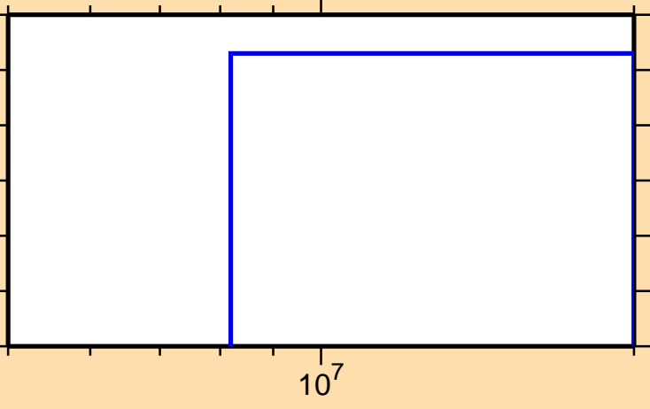
\sigma vs. E for ^{200}\text{Po}(n,2np)
