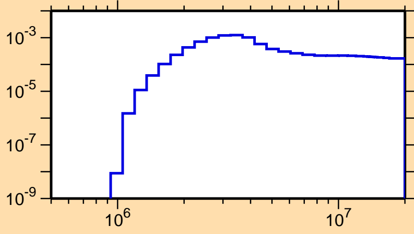
\sigma vs. E for ^{201}\text{Po}(n,n_4)
