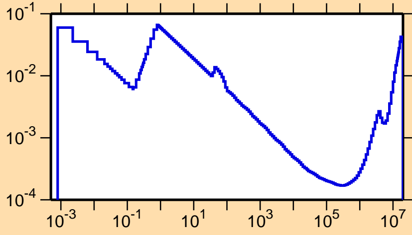
\sigma vs. E for ^{201}\text{Po}(n,\alpha)
