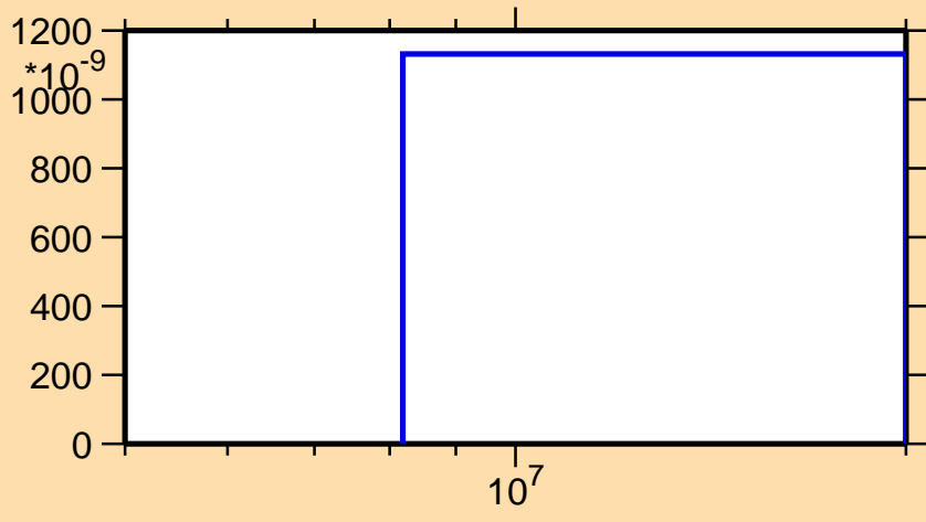
\sigma vs. E for ^{201}\text{Po}(n,2n\alpha)
