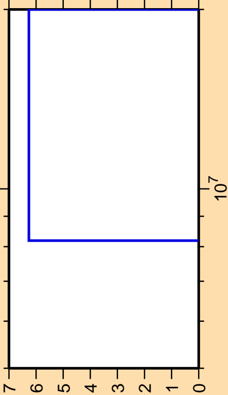
\Delta\sigma/\sigma vs. E for ^{201}\text{Po}(\text{mt } 34)
