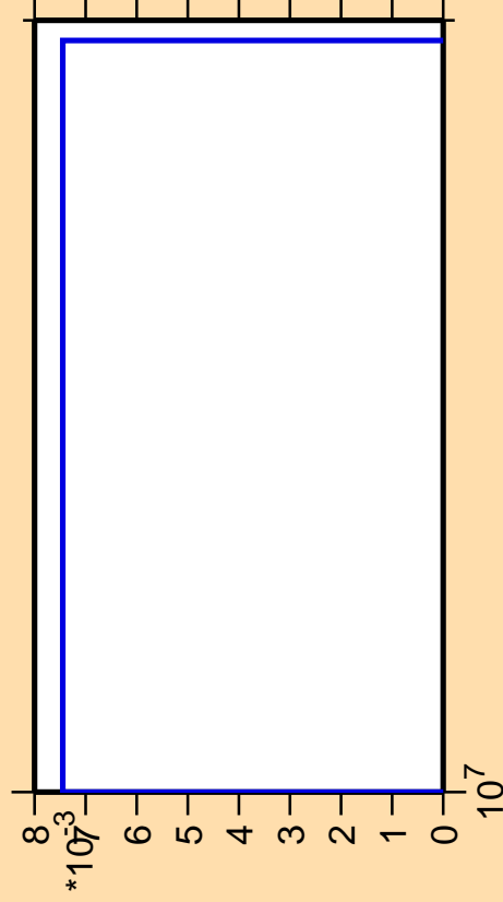
\Delta\sigma/\sigma vs. E for ^{201}\text{Po}(n,3n\alpha)
