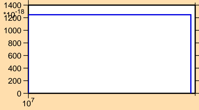
\sigma vs. E for ^{201}\text{Po}(n,3n\alpha)
