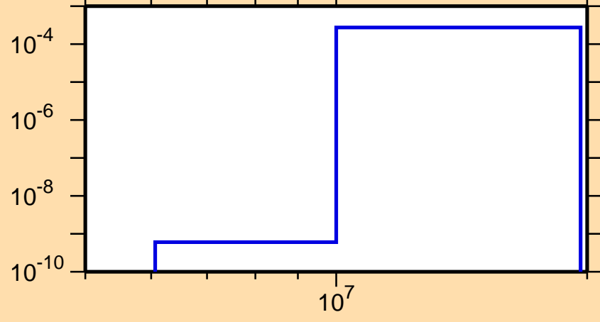
\sigma vs. E for ^{201}\text{Po}(n,t)
