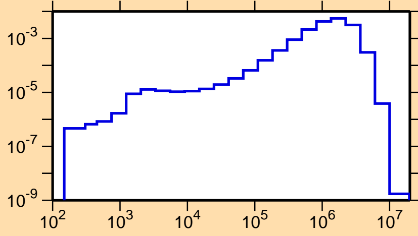
\sigma vs. E for ^{201}\text{Po}(n,n_1)
