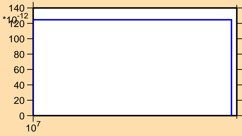
\sigma vs. E for ^{201}\text{Po} (mt 45)
