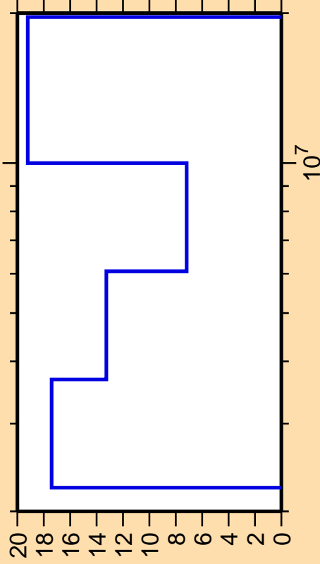
\Delta\sigma/\sigma vs. E for ^{202}\text{Po}(n,n\text{cont.})
