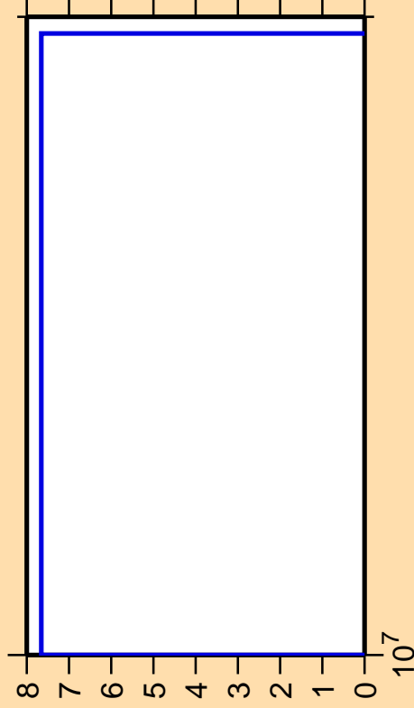
\Delta\sigma/\sigma vs. E for ^{202}\text{Po}(n,\text{pt})
