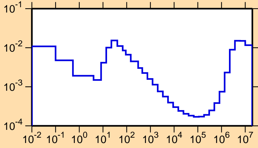
\sigma vs. E for ^{202}\text{Po}(n,\alpha)
