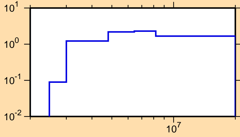
\sigma vs. E for ^{202}\text{Po}(n,n\text{cont.})
