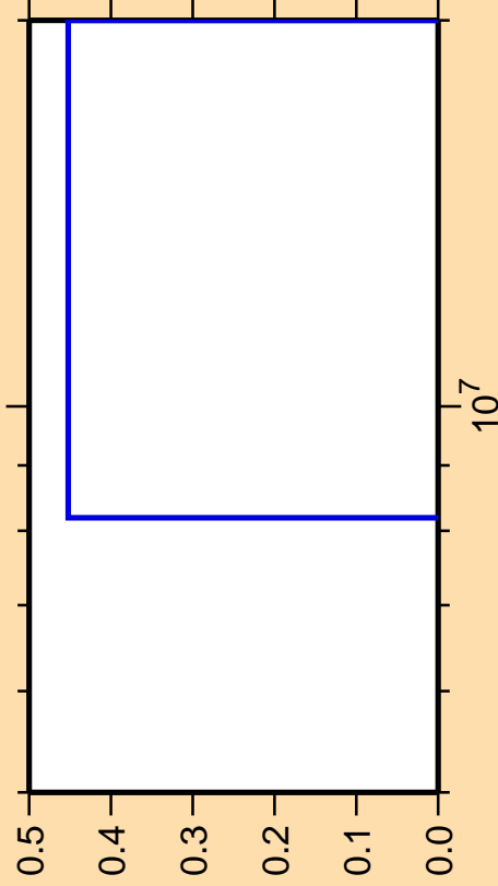
\Delta\sigma/\sigma vs. E for ^{202}\text{Po} (mt 34)
