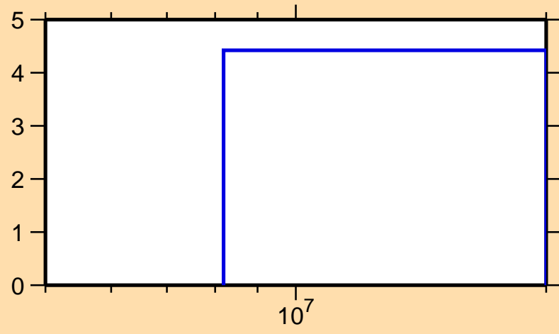
\Delta\sigma/\sigma vs. E for ^{202}\text{Po}(n,\text{el.})
