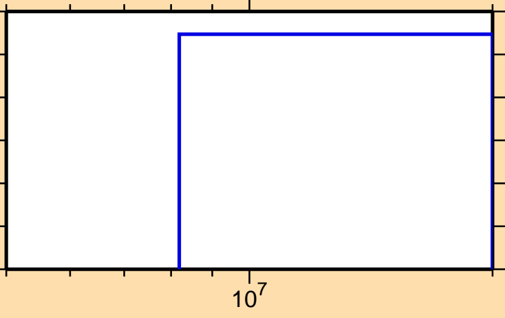
\sigma vs. E for ^{202}\text{Po}(n,nt)
