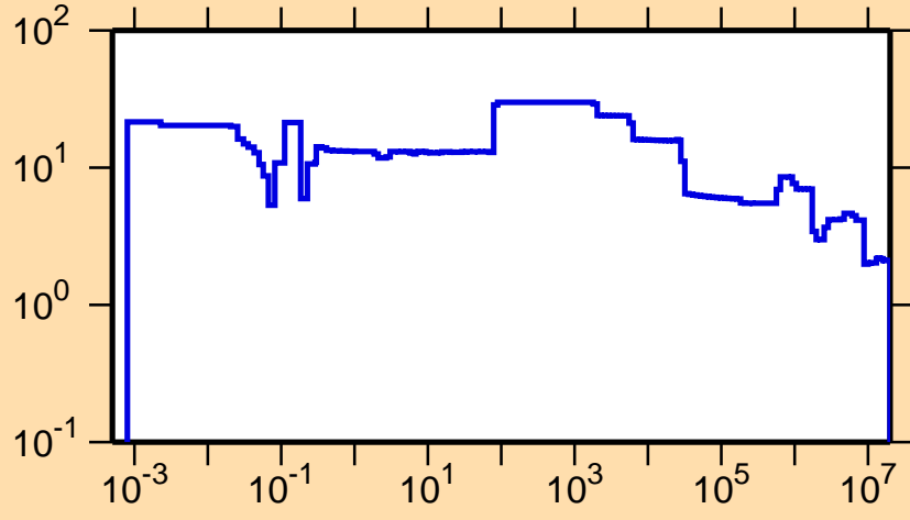
\Delta\sigma/\sigma vs. E for ^{203}\text{Po}(n,\text{tot.})
