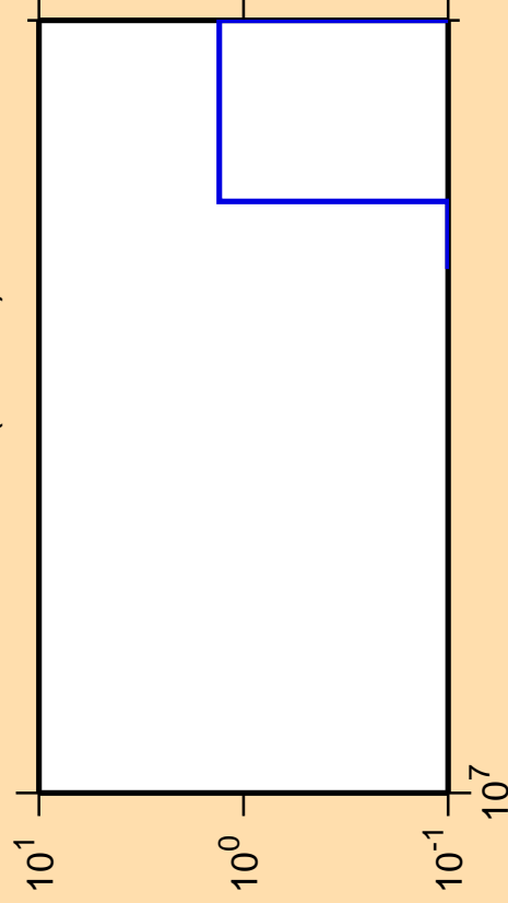
\Delta\sigma/\sigma vs. E for ^{203}\text{Po}(n,3n\alpha)
