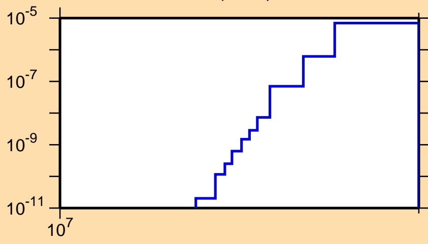
\sigma vs. E for ^{203}\text{Po}(n,\text{nd})
