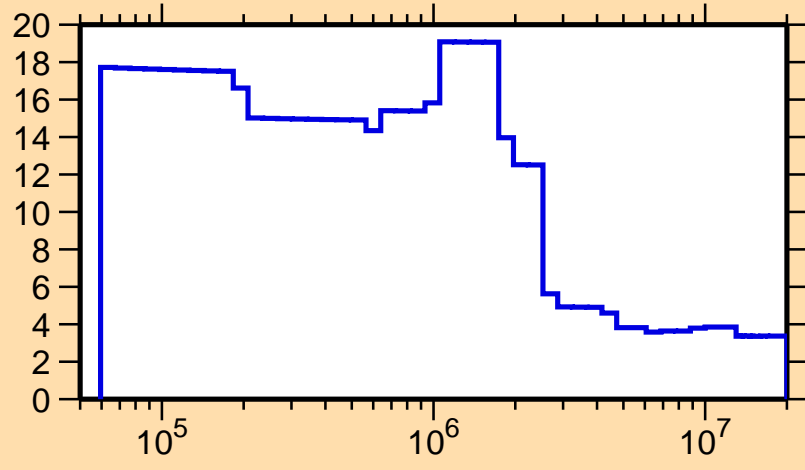
\Delta\sigma/\sigma vs. E for ^{203}\text{Po}(n,\text{nonel.})
