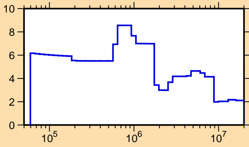
\Delta\sigma/\sigma vs. E for ^{203}\text{Po}(n,\text{tot.})
