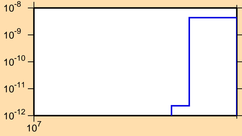
\sigma vs. E for ^{203}\text{Po}(n,nt)
