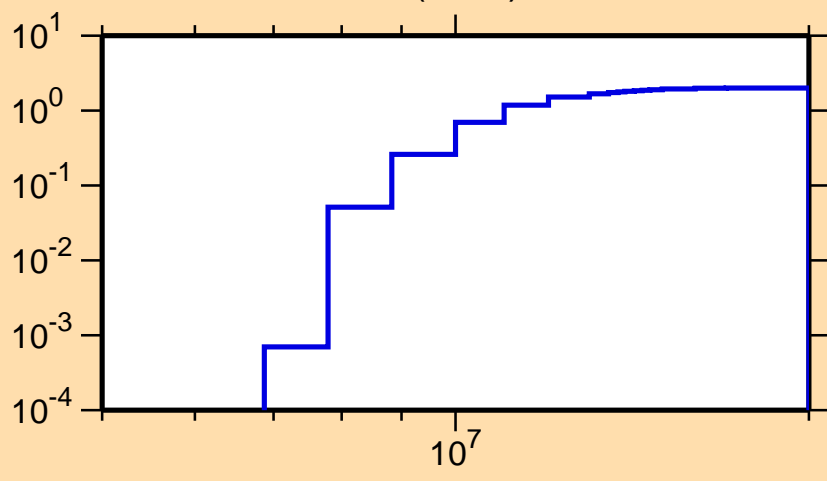
\sigma vs. E for ^{203}\text{Po}(n,2n)
