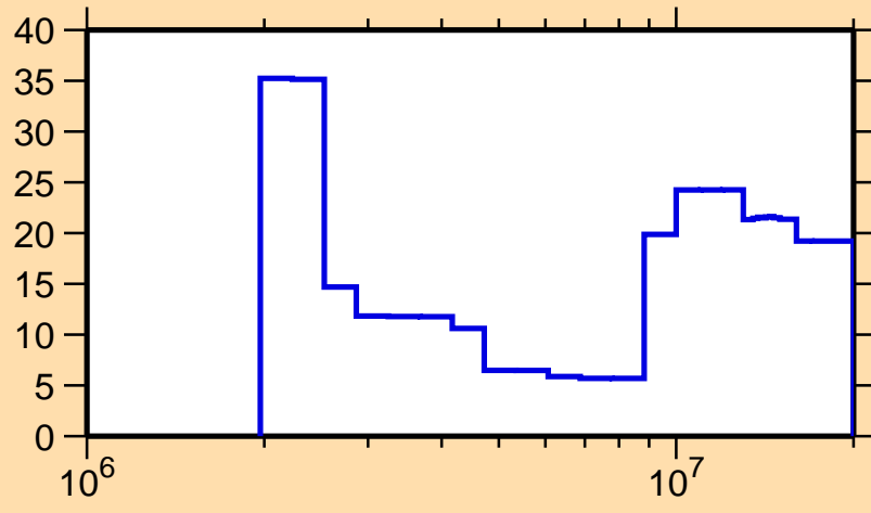
\Delta\sigma/\sigma vs. E for ^{203}\text{Po}(n,n\text{cont.})
