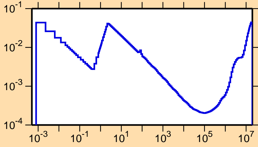
\sigma vs. E for ^{203}\text{Po}(n,p)
