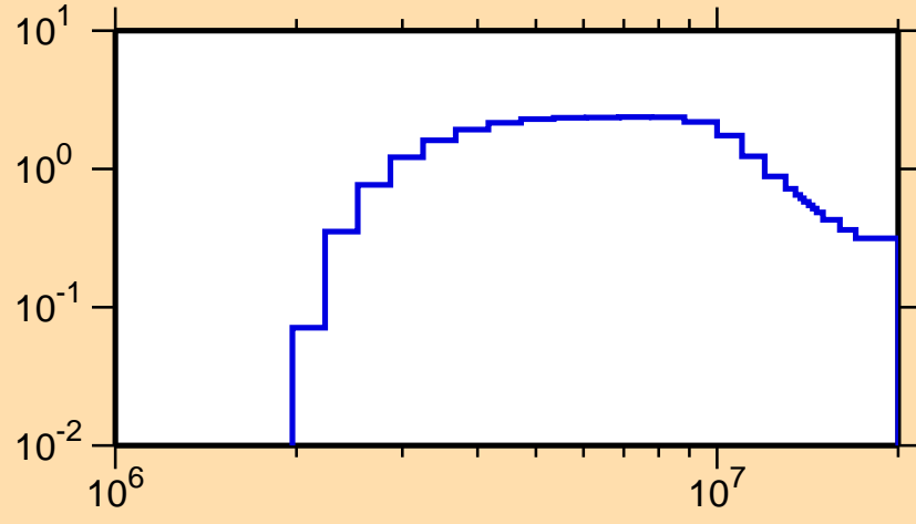
\sigma vs. E for ^{203}\text{Po}(n,n\text{cont.})
