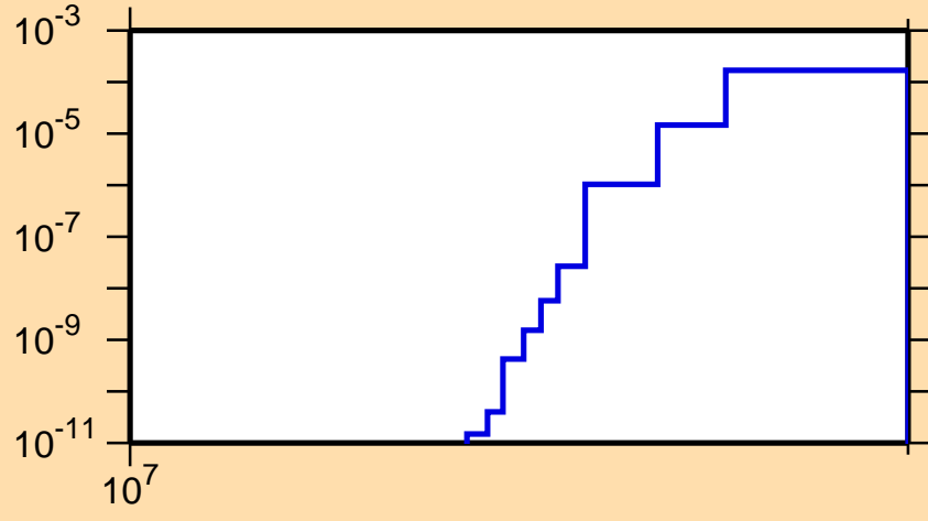
\sigma vs. E for ^{203}\text{Po}(n,2np)
