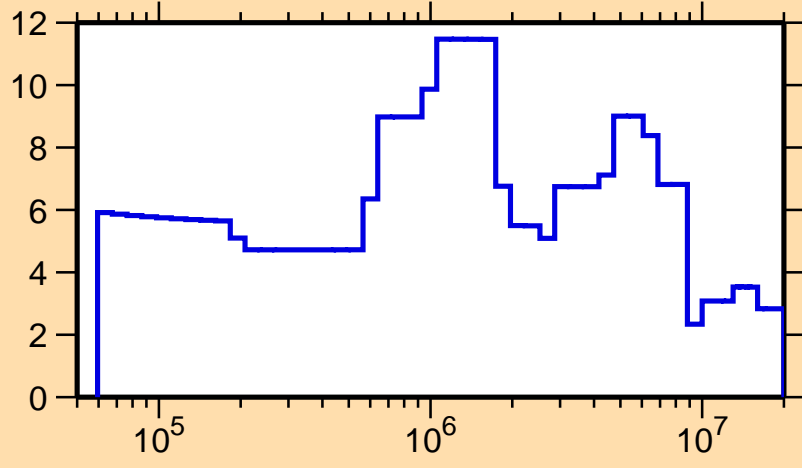
\Delta\sigma/\sigma vs. E for ^{203}\text{Po}(n,\text{el.})
