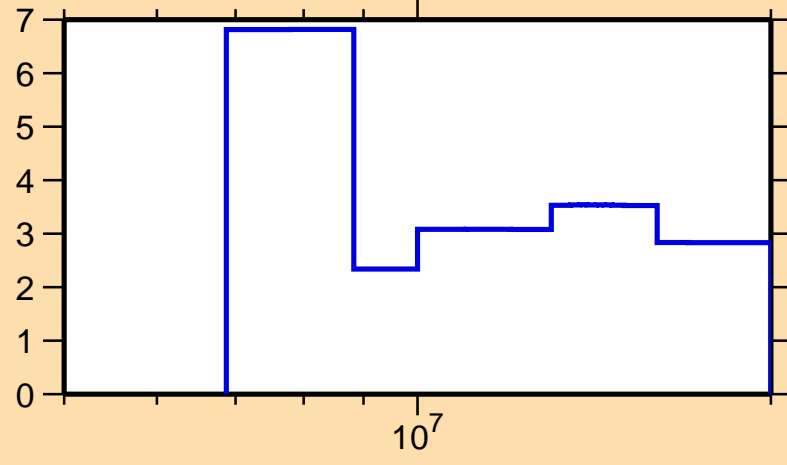
\Delta\sigma/\sigma vs. E for ^{203}\text{Po}(n,\text{el.})
