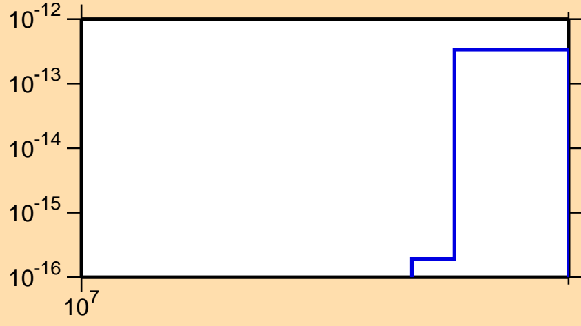
\sigma vs. E for ^{203}\text{Po}(n,3n\alpha)
