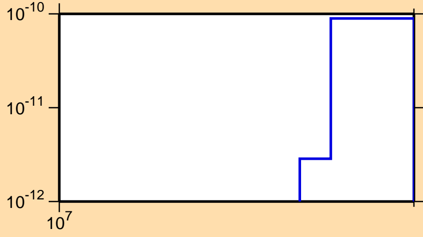
\sigma vs. E for ^{203}\text{Po} (mt 34)
