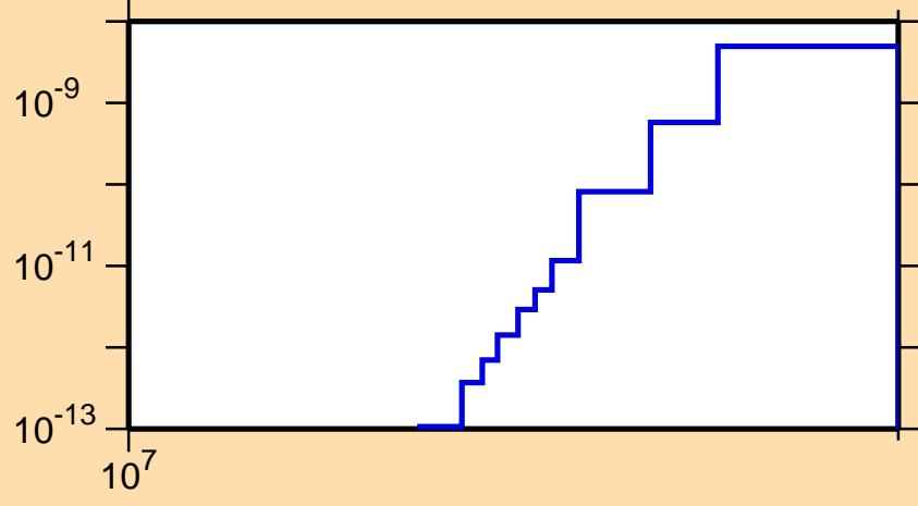
\sigma vs. E for ^{203}\text{Po}(n,pd)
