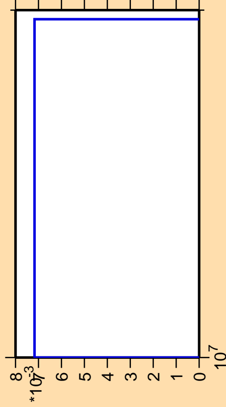
\Delta\sigma/\sigma vs. E for ^{203}\text{Po}(n,3n\alpha)
