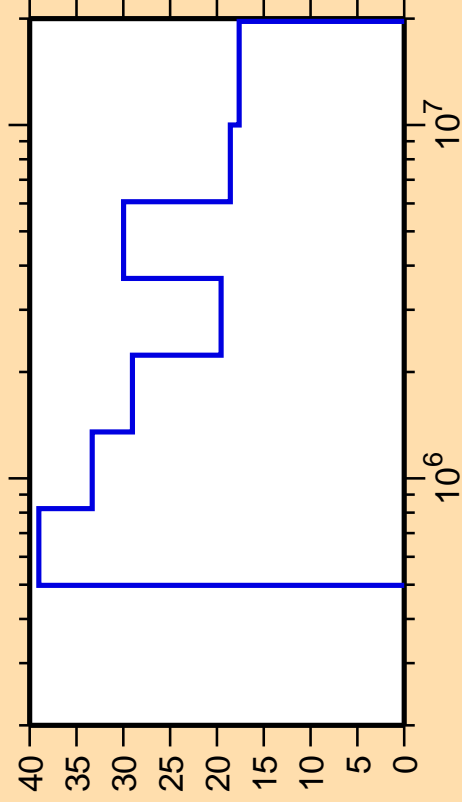
\Delta\sigma/\sigma vs. E for ^{203}\text{Po}(n,n_4)
