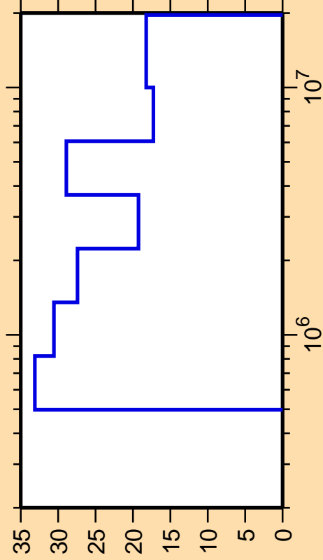
\Delta\sigma/\sigma vs. E for ^{203}\text{Po}(n,n_3)
