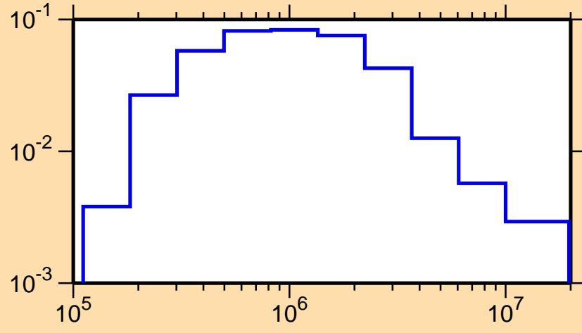
\sigma vs. E for ^{203}\text{Po}(n,n_2)
