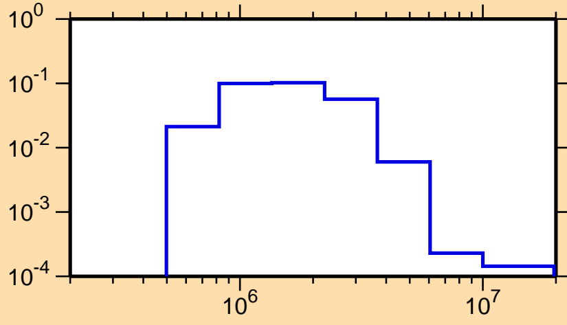
\sigma vs. E for ^{203}\text{Po}(n,n_4)
