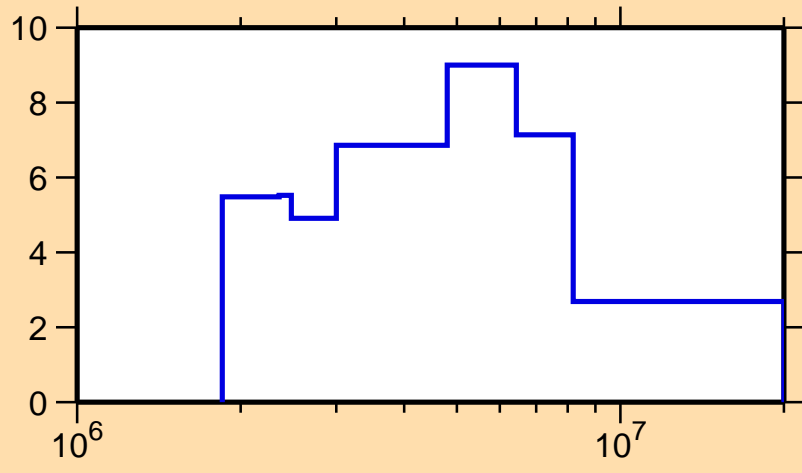
\Delta\sigma/\sigma vs. E for ^{203}\text{Po}(n, el.)
