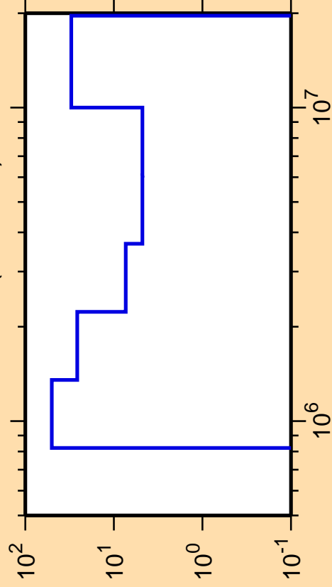
\Delta\sigma/\sigma vs. E for ^{203}\text{Po}(n,\text{ncont.})
