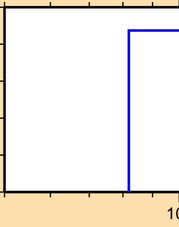
\sigma vs. E for ^{203}\text{Po}(n,2np)
