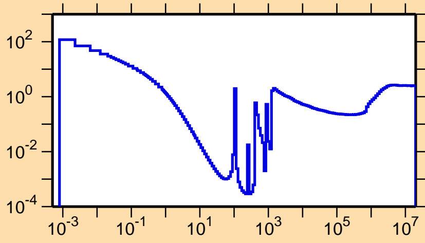
\sigma vs. E for ^{204}\text{Po}(n,\text{nonel.})
