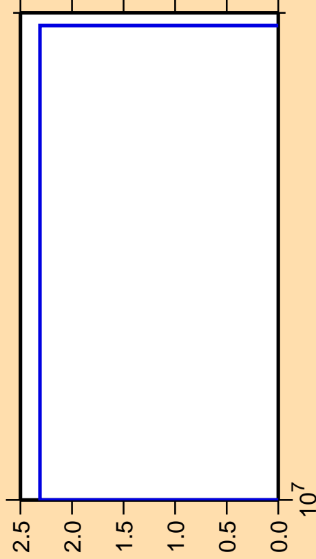
\Delta\sigma/\sigma vs. E for ^{204}\text{Po}(\text{mt } 45)
