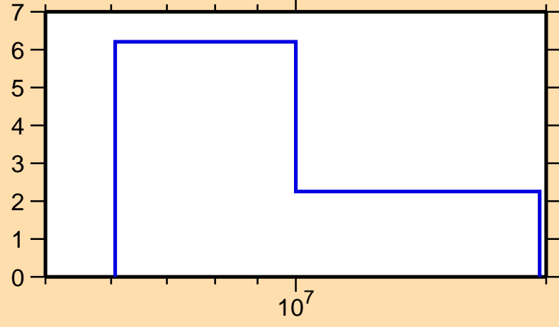
\Delta\sigma/\sigma vs. E for ^{204}\text{Po}(n,\text{el.})
