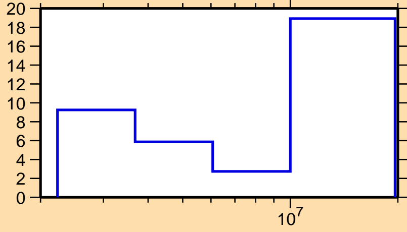
\Delta\sigma/\sigma vs. E for ^{204}\text{Po}(n,n\text{cont.})
