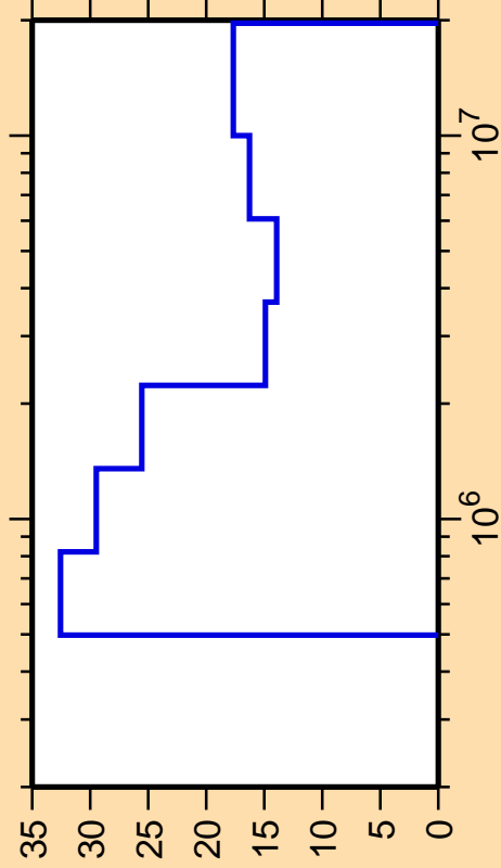
\Delta\sigma/\sigma vs. E for ^{204}\text{Po}(n,n_1)
