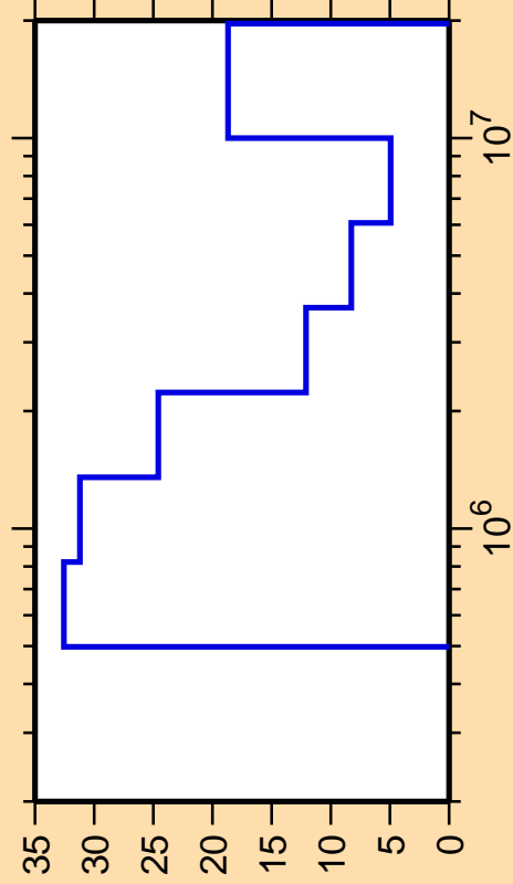
\Delta\sigma/\sigma vs. E for ^{204}\text{Po}(n,\text{inel.})
