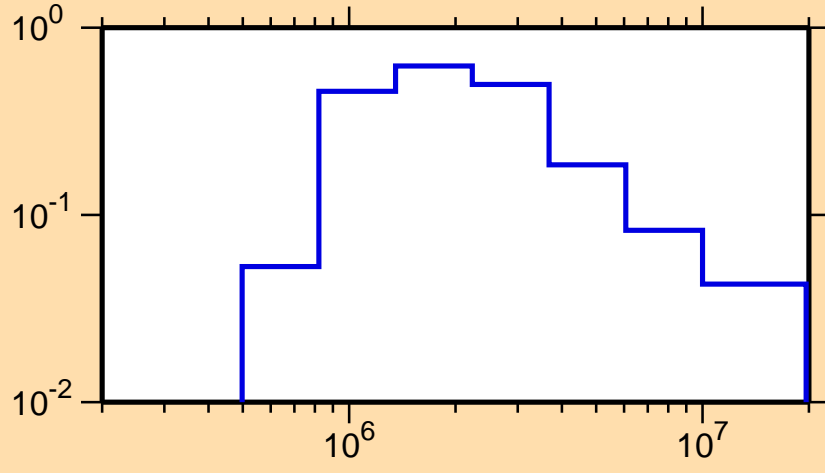
\sigma vs. E for ^{204}\text{Po}(n,n_1)
