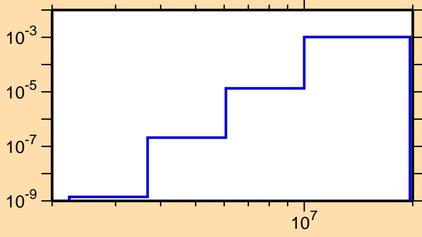
\sigma vs. E for ^{204}\text{Po}(n,n\alpha)
